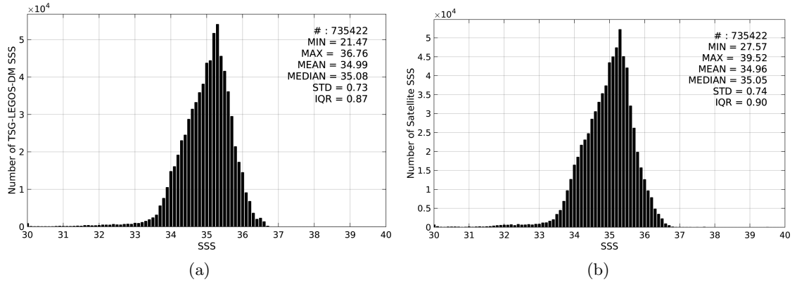
Figure 2: Histograms of SSS from TSG-LEGOS-DM (a) and SMOS-L3-CATDS-CPDC-V3-MONTHLY-25KM (b) considering all match-up pairs per bins of 0.1 over the Tropical Pacific Ocean Pi-MEP region and for the full satellite product period.
