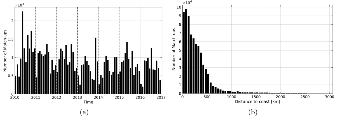
Figure 1: Number of match-ups between TSG-LEGOS-DM and SMOS-L3-CATDS-CPDC-V3-MONTHLY-25KM SSS as a function of time (a) and as function of the distance to coast (b) over the Tropical Pacific Ocean Pi-MEP region and for the full satellite product period.
