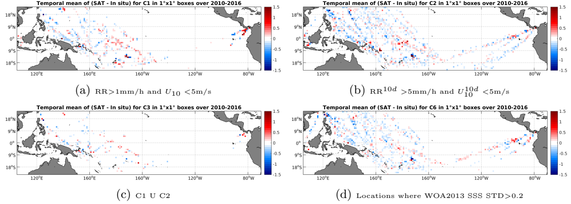
Figure 12: Temporal mean gridded over spatial boxes of size 1^\circ \times 1^\circ of \Delta SSS (SMOS-L3-CATDS-CPDC-V3-MONTHLY-25KM - TSG-LEGOS-DM) for 4 different subdatasets corresponding to: RR > 1\text{mm/h} and U_{10} < 5\text{m/s} (a), RR^{10d} > 5\text{mm/h} and U_{10}^{10d} < 5\text{m/s} (b), C1 U C2 (c), Locations where WOA2013 SSS STD > 0.2 (d).
