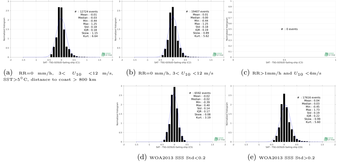
Figure 13: Normalized histogram of \Delta SSS (SMOS-L3-CATDS-CPDC-V3-MONTHLY-25KM - TSG-GOSUD-Sailing-ship) for 5 different subdatasets corresponding to: RR=0 mm/h, 3 < U_{10} < 12 m/s, SST > 5^\circ C , distance to coast > 800 km (a), RR=0 mm/h, 3 < U_{10} < 12 m/s (b), RR > 1 mm/h and U_{10} < 4 m/s (c), WOA2013 SSS Std < 0.2 (d), WOA2013 SSS Std > 0.2 (e).
