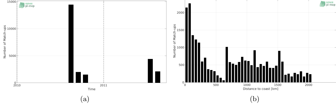
Figure 1: Number of match-ups between TSG-GOSUD-Sailing-ship and SMOS-L3-CATDS-CPDC-V3-MONTHLY-25KM SSS as a function of time (a) and as function of the distance to coast (b) over the Tropical Pacific Ocean Pi-MEP region and for the full satellite product period.
