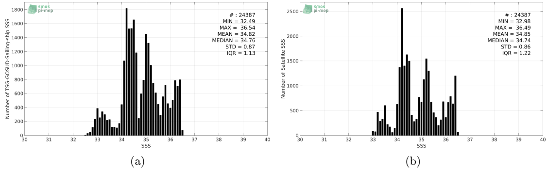
Figure 2: Histograms of SSS from TSG-GOSUD-Sailing-ship (a) and SMOS-L3-CATDS-CPDC-V3-MONTHLY-25KM (b) considering all match-up pairs per bins of 0.1 over the Tropical Pacific Ocean Pi-MEP region and for the full satellite product period.
