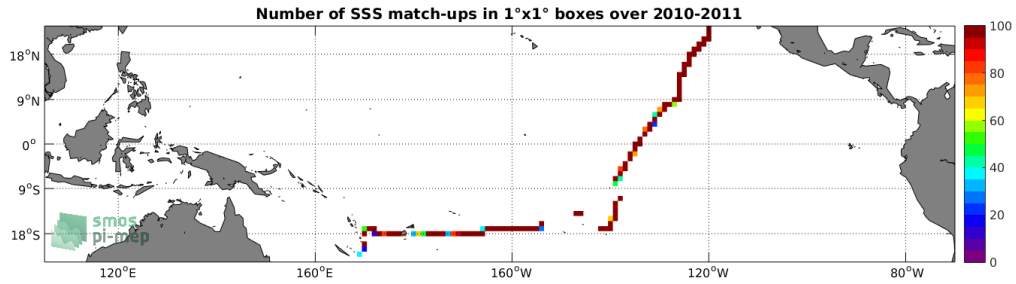
Figure 4: Number of SSS match-ups between TSG-GOSUD-Sailing-ship SSS and the SMOS-L3-CATDS-CPDC-V3-MONTHLY-25KM SSS product for the Tropical Pacific Ocean Pi-MEP region over 1^\circ \times 1^\circ boxes and for the full satellite product period.
