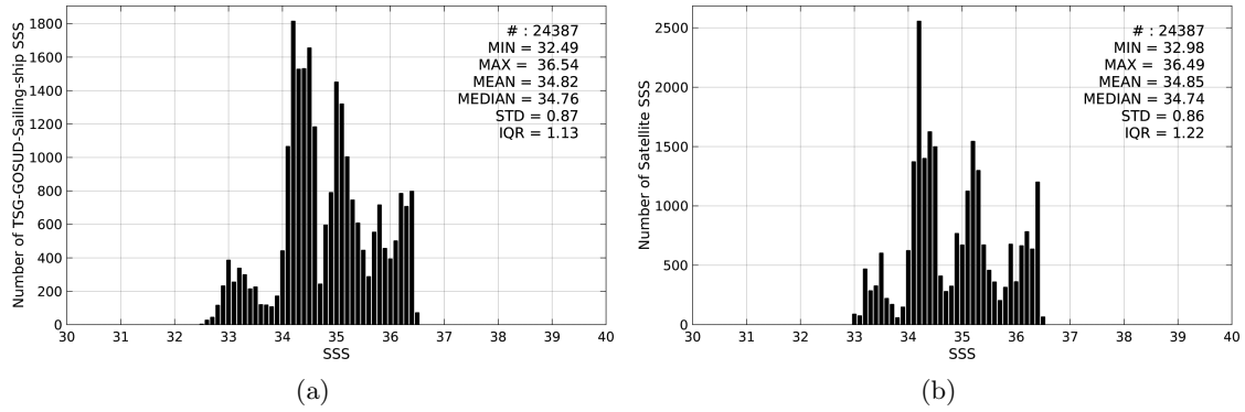
Figure 2: Histograms of SSS from TSG-GOSUD-Sailing-ship (a) and SMOS-L3-CATDS-CPDC-V3-MONTHLY-25KM (b) considering all match-up pairs per bins of 0.1 over the Tropical Pacific Ocean Pi-MEP region and for the full satellite product period.
