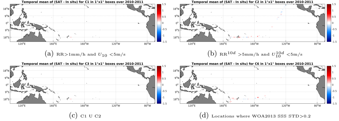
Figure 12: Temporal mean gridded over spatial boxes of size 1^\circ \times 1^\circ of \Delta SSS (SMOS-L3-CATDS-CPDC-V3-MONTHLY-25KM - TSG-GOSUD-Sailing-ship) for 4 different subdatasets corresponding to: RR > 1mm/h and U_{10} < 5 m/s (a), RR^{10d} > 5 mm/h and U_{10}^{10d} < 5 m/s (b), C1 U C2 (c), Locations where WOA2013 SSS STD > 0.2 (d).
