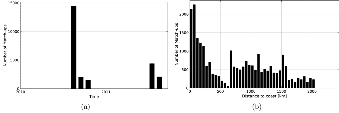
Figure 1: Number of match-ups between TSG-GOSUD-Sailing-ship and SMOS-L3-CATDS-CPDC-V3-MONTHLY-25KM SSS as a function of time (a) and as function of the distance to coast (b) over the Tropical Pacific Ocean Pi-MEP region and for the full satellite product period.
