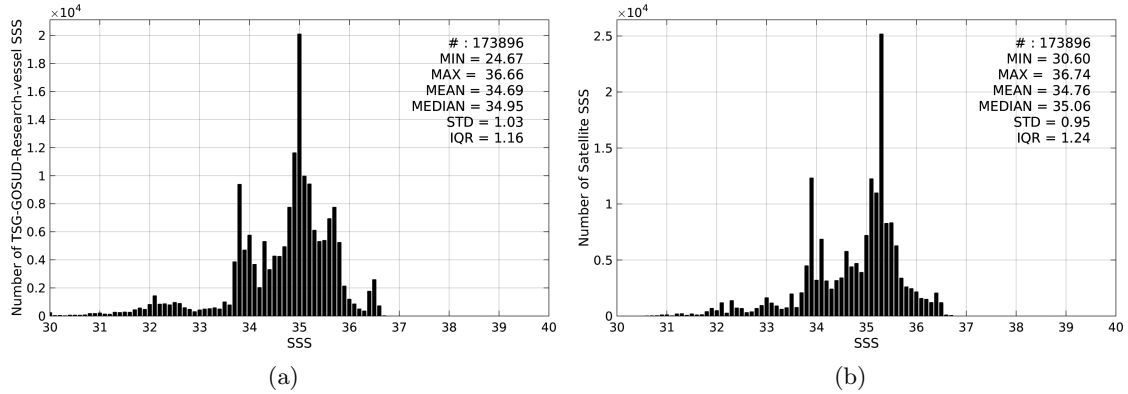
Figure 2: Histograms of SSS from TSG-GOSUD-Research-vessel (a) and SMOS-L3-CATDS-CPDC-V3-MONTHLY-25KM (b) considering all match-up pairs per bins of 0.1 over the Tropical Pacific Ocean Pi-MEP region and for the full satellite product period.
