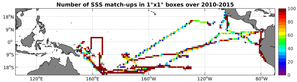
Figure 4: Number of SSS match-ups between TSG-GOSUD-Research-vessel SSS and the SMOS-L3-CATDS-CPDC-V3-MONTHLY-25KM SSS product for the Tropical Pacific Ocean Pi-MEP region over 1^\circ \times 1^\circ boxes and for the full satellite product period.
