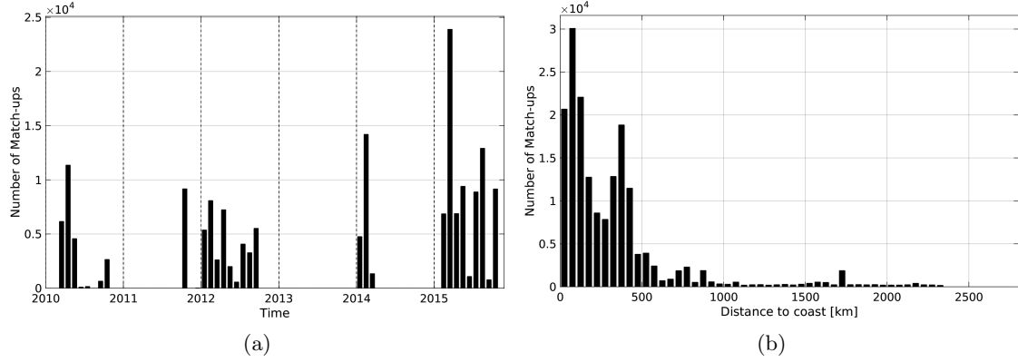
Figure 1: Number of match-ups between TSG-GOSUD-Research-vessel and SMOS-L3-CATDS-CPDC-V3-MONTHLY-25KM SSS as a function of time (a) and as function of the distance to coast (b) over the Tropical Pacific Ocean Pi-MEP region and for the full satellite product period.
