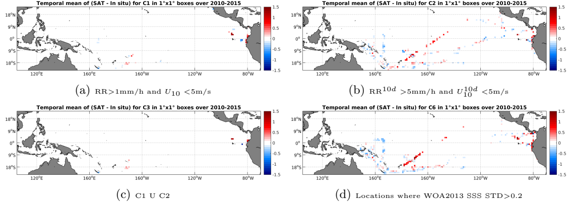
Figure 12: Temporal mean gridded over spatial boxes of size 1^\circ \times 1^\circ of \Delta SSS (SMOS-L3-CATDS-CPDC-V3-MONTHLY-25KM - TSG-GOSUD-Research-vessel) for 4 different subdatasets corresponding to: RR > 1\text{mm/h} and U_{10} < 5\text{m/s} (a), RR^{10d} > 5\text{mm/h} and U_{10}^{10d} < 5\text{m/s} (b), C1 U C2 (c), Locations where WOA2013 SSS STD > 0.2 (d).
