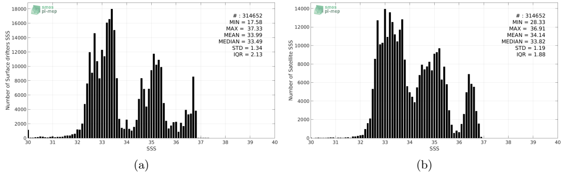
Figure 2: Histograms of SSS from Surface drifters (a) and SMOS-L3-CATDS-CPDC-V3-MONTHLY-25KM (b) considering all match-up pairs per bins of 0.1 over the Tropical Pacific Ocean Pi-MEP region and for the full satellite product period.
