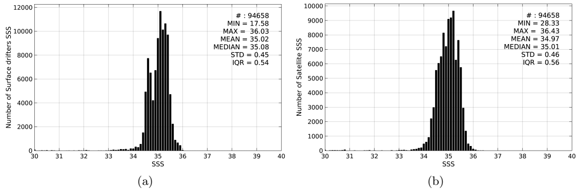
Figure 2: Histograms of SSS from Surface drifters (a) and SMOS-L3-CATDS-CPDC-V3-MONTHLY-25KM (b) considering all match-up pairs per bins of 0.1 over the Tropical Pacific Ocean Pi-MEP region and for the full satellite product period.
