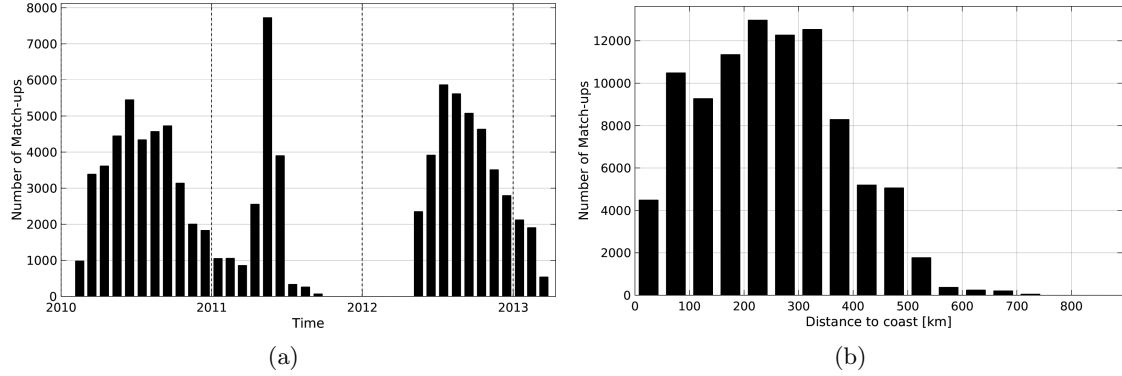
Figure 1: Number of match-ups between Surface drifters and SMOS-L3-CATDS-CPDC-V3-MONTHLY-25KM SSS as a function of time (a) and as function of the distance to coast (b) over the Tropical Pacific Ocean Pi-MEP region and for the full satellite product period.
