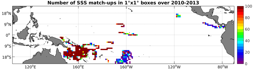
Figure 3: Number of SSS match-ups between Surface drifters SSS and the SMOS-L3-CATDS-CPDC-V3-MONTHLY-25KM SSS product for the Tropical Pacific Ocean Pi-MEP region over 1^\circ \times 1^\circ boxes and for the full satellite product period.
