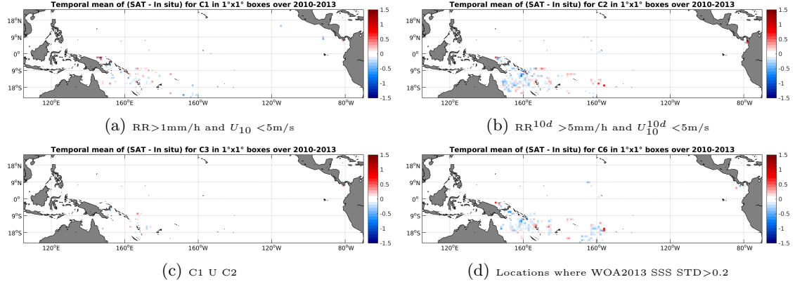
Figure 11: Temporal mean gridded over spatial boxes of size 1^\circ \times 1^\circ of \Delta SSS (SMOS-L3-CATDS-CPDC-V3-MONTHLY-25KM - Surface drifters) for 4 different subdatasets corresponding to: RR > 1mm/h and U_{10} < 5 m/s (a), RR^{10d} > 5 mm/h and U_{10}^{10d} < 5 m/s (b), C1 U C2 (c), Locations where WOA2013 SSS STD > 0.2 (d).
