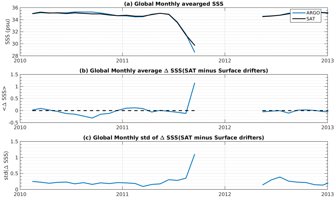
Figure 6: Time series of the monthly averaged mean SSS (top), mean \Delta SSS (Satellite - Surface drifters) and STD of \Delta SSS (Satellite - Surface drifters) over the Tropical Pacific Ocean Pi-MEP region considering all match-ups collected by the Pi-MEP platform.
