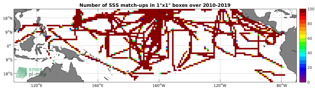
Figure 4: Number of SSS match-ups between TSG-SAMOS SSS and the SMOS-L3-CATDS-CPDC-V3-10DAYS-25KM SSS product for the Tropical Pacific Ocean Pi-MEP region over 1^\circ \times 1^\circ boxes and for the full satellite product period.
