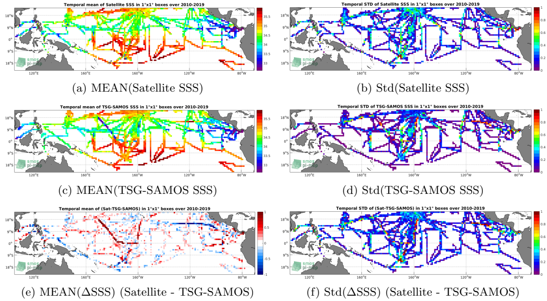
Figure 6: Temporal mean (left) and Std (right) of SSS from SMOS-L3-CATDS-CPDC-V3-10DAYS-25KM (top), TSG-SAMOS (middle), and of \Delta SSS (Satellite - TSG-SAMOS). Only match-up pairs are used to generate these maps.
