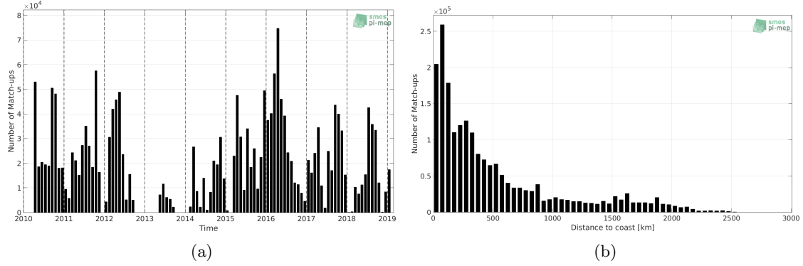
Figure 1: Number of match-ups between TSG-SAMOS and SMOS-L3-CATDS-CPDC-V3-10DAYS-25KM SSS as a function of time (a) and as function of the distance to coast (b) over the Tropical Pacific Ocean Pi-MEP region and for the full satellite product period.
