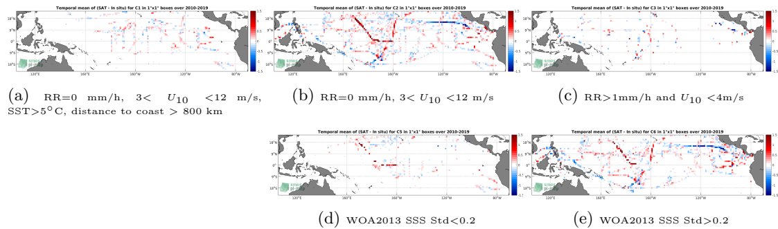
Figure 12: Temporal mean gridded over spatial boxes of size 1^\circ \times 1^\circ of \Delta SSS (SMOS-L3-CATDS-CPDC-V3-10DAYS-25KM - TSG-SAMOS) for 5 different subdatasets corresponding to:RR=0 mm/h, 3 < U_{10} < 12 m/s, SST > 5^\circ\text{C} , distance to coast > 800 km (a), RR=0 mm/h, 3 < U_{10} < 12 m/s (b), RR > 1 mm/h and U_{10} < 4 m/s (c), WOA2013 SSS Std < 0.2 (d), WOA2013 SSS Std > 0.2 (e).
