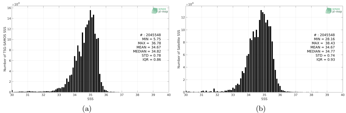
Figure 2: Histograms of SSS from TSG-SAMOS (a) and SMOS-L3-CATDS-CPDC-V3-10DAYS-25KM (b) considering all match-up pairs per bins of 0.1 over the Tropical Pacific Ocean Pi-MEP region and for the full satellite product period.
