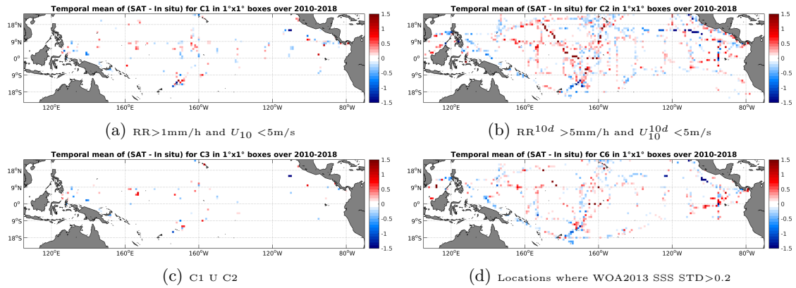
Figure 12: Temporal mean gridded over spatial boxes of size 1^\circ \times 1^\circ of \Delta SSS (SMOS-L3-CATDS-CPDC-V3-10DAYS-25KM - TSG-SAMOS) for 4 different subdatasets corresponding to: RR > 1\text{mm/h} and U_{10} < 5\text{m/s} (a), RR^{10d} > 5\text{mm/h} and U_{10}^{10d} < 5\text{m/s} (b), C1 U C2 (c), Locations where WOA2013 SSS STD > 0.2 (d).
