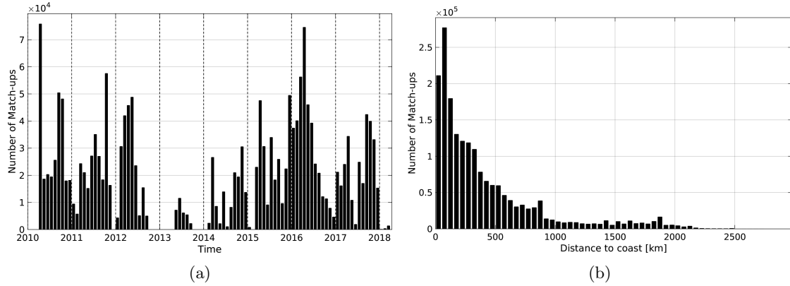
Figure 1: Number of match-ups between TSG-SAMOS and SMOS-L3-CATDS-CPDC-V3-10DAYS-25KM SSS as a function of time (a) and as function of the distance to coast (b) over the Tropical Pacific Ocean Pi-MEP region and for the full satellite product period.
