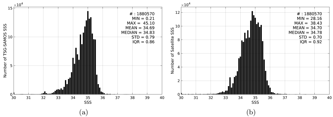
Figure 2: Histograms of SSS from TSG-SAMOS (a) and SMOS-L3-CATDS-CPDC-V3-10DAYS-25KM (b) considering all match-up pairs per bins of 0.1 over the Tropical Pacific Ocean Pi-MEP region and for the full satellite product period.
