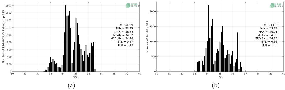
Figure 2: Histograms of SSS from TSG-GOSUD-Sailing-ship (a) and SMOS-L3-CATDS-CPDC-V3-10DAYS-25KM (b) considering all match-up pairs per bins of 0.1 over the Tropical Pacific Ocean Pi-MEP region and for the full satellite product period.
