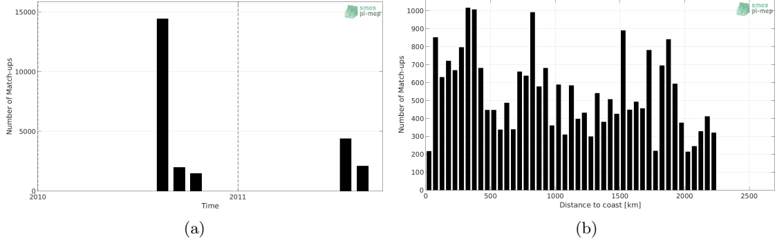
Figure 1: Number of match-ups between TSG-GOSUD-Sailing-ship and SMOS-L3-CATDS-CPDC-V3-10DAYS-25KM SSS as a function of time (a) and as function of the distance to coast (b) over the Tropical Pacific Ocean Pi-MEP region and for the full satellite product period.
