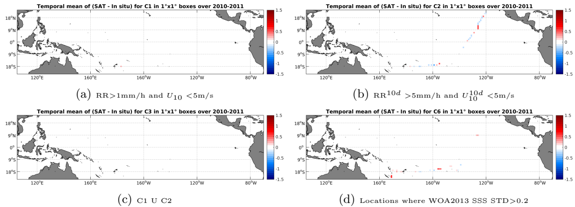
Figure 12: Temporal mean gridded over spatial boxes of size 1^\circ \times 1^\circ of \Delta SSS (SMOS-L3-CATDS-CPDC-V3-10DAYS-25KM - TSG-GOSUD-Sailing-ship) for 4 different subdatasets corresponding to: RR > 1\text{mm/h} and U_{10} < 5\text{m/s} (a), RR^{10d} > 5\text{mm/h} and U_{10}^{10d} < 5\text{m/s} (b), C1 U C2 (c), Locations where WOA2013 SSS STD > 0.2 (d).
