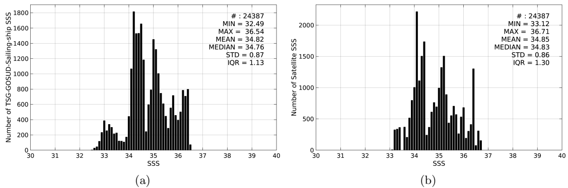
Figure 2: Histograms of SSS from TSG-GOSUD-Sailing-ship (a) and SMOS-L3-CATDS-CPDC-V3-10DAYS-25KM (b) considering all match-up pairs per bins of 0.1 over the Tropical Pacific Ocean Pi-MEP region and for the full satellite product period.
