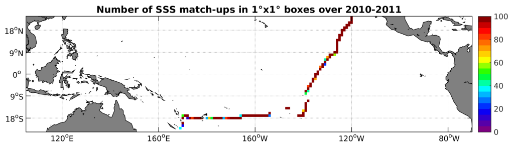
Figure 4: Number of SSS match-ups between TSG-GOSUD-Sailing-ship SSS and the SMOS-L3-CATDS-CPDC-V3-10DAYS-25KM SSS product for the Tropical Pacific Ocean Pi-MEP region over 1^\circ \times 1^\circ boxes and for the full satellite product period.
