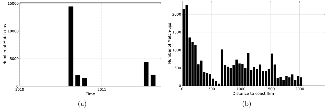
Figure 1: Number of match-ups between TSG-GOSUD-Sailing-ship and SMOS-L3-CATDS-CPDC-V3-10DAYS-25KM SSS as a function of time (a) and as function of the distance to coast (b) over the Tropical Pacific Ocean Pi-MEP region and for the full satellite product period.
