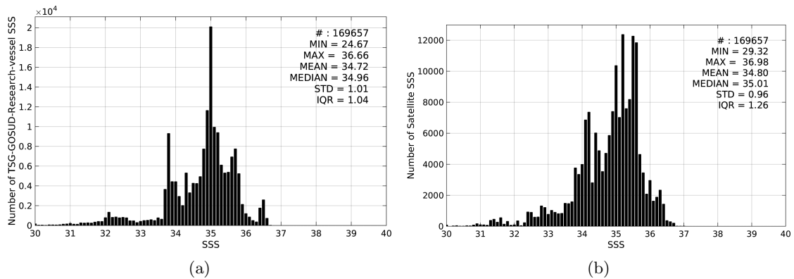
Figure 2: Histograms of SSS from TSG-GOSUD-Research-vessel (a) and SMOS-L3-CATDS-CPDC-V3-10DAYS-25KM (b) considering all match-up pairs per bins of 0.1 over the Tropical Pacific Ocean Pi-MEP region and for the full satellite product period.
