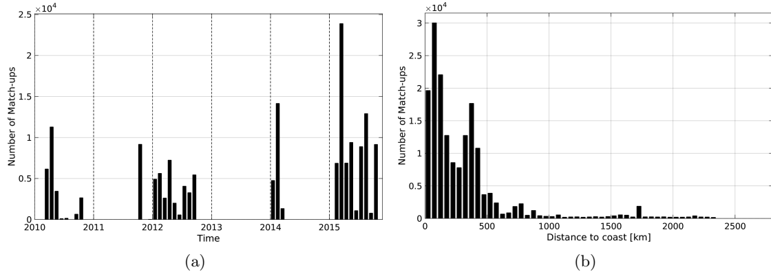
Figure 1: Number of match-ups between TSG-GOSUD-Research-vessel and SMOS-L3-CATDS-CPDC-V3-10DAYS-25KM SSS as a function of time (a) and as function of the distance to coast (b) over the Tropical Pacific Ocean Pi-MEP region and for the full satellite product period.
