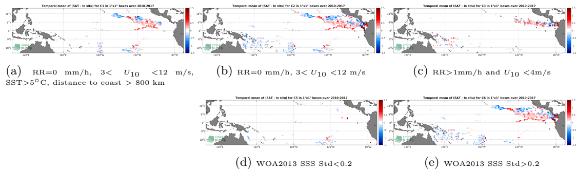
Figure 11: Temporal mean gridded over spatial boxes of size 1^\circ \times 1^\circ of \Delta SSS (SMOS-L3-CATDS-CPDC-V3-10DAYS-25KM - Surface drifters) for 5 different subdatasets corresponding to:RR=0 mm/h, 3 < U_{10} < 12 m/s, SST > 5^\circ\text{C} , distance to coast > 800 km (a), RR=0 mm/h, 3 < U_{10} < 12 m/s (b), RR > 1 mm/h and U_{10} < 4 m/s (c), WOA2013 SSS Std < 0.2 (d), WOA2013 SSS Std > 0.2 (e).
