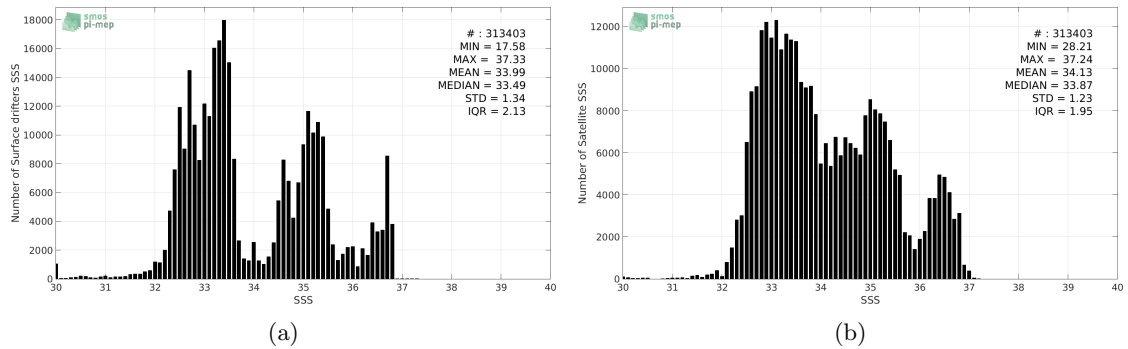
Figure 2: Histograms of SSS from Surface drifters (a) and SMOS-L3-CATDS-CPDC-V3-10DAYS-25KM (b) considering all match-up pairs per bins of 0.1 over the Tropical Pacific Ocean Pi-MEP region and for the full satellite product period.
