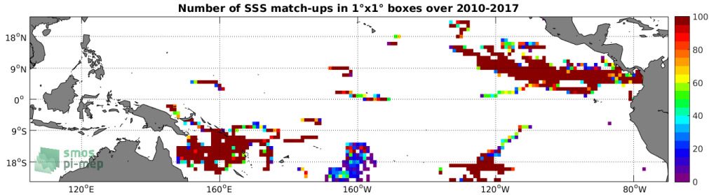
Figure 3: Number of SSS match-ups between Surface drifters SSS and the SMOS-L3-CATDS-CPDC-V3-10DAYS-25KM SSS product for the Tropical Pacific Ocean Pi-MEP region over 1^\circ \times 1^\circ boxes and for the full satellite product period.
