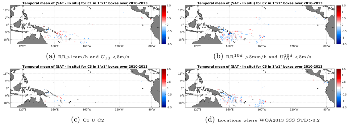
Figure 11: Temporal mean gridded over spatial boxes of size 1^\circ \times 1^\circ of \Delta SSS (SMOS-L3-CATDS-CPDC-V3-10DAYS-25KM - Surface drifters) for 4 different subdatasets corresponding to: RR > 1\text{mm/h} and U_{10} < 5\text{m/s} (a), RR^{10d} > 5\text{mm/h} and U_{10}^{10d} < 5\text{m/s} (b), C1 U C2 (c), Locations where WOA2013 SSS STD > 0.2 (d).
