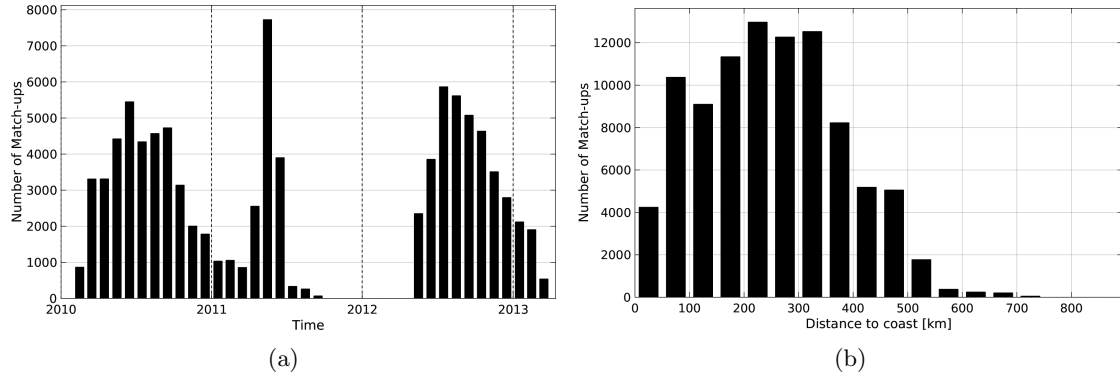
Figure 1: Number of match-ups between Surface drifters and SMOS-L3-CATDS-CPDC-V3-10DAYS-25KM SSS as a function of time (a) and as function of the distance to coast (b) over the Tropical Pacific Ocean Pi-MEP region and for the full satellite product period.
