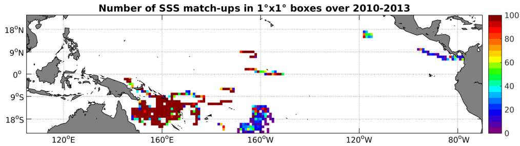
Figure 3: Number of SSS match-ups between Surface drifters SSS and the SMOS-L3-CATDS-CPDC-V3-10DAYS-25KM SSS product for the Tropical Pacific Ocean Pi-MEP region over 1^\circ \times 1^\circ boxes and for the full satellite product period.
