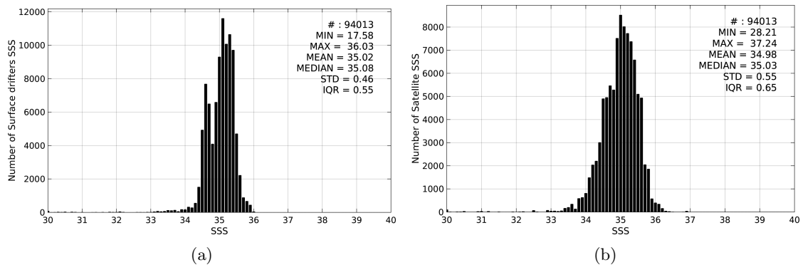
Figure 2: Histograms of SSS from Surface drifters (a) and SMOS-L3-CATDS-CPDC-V3-10DAYS-25KM (b) considering all match-up pairs per bins of 0.1 over the Tropical Pacific Ocean Pi-MEP region and for the full satellite product period.
