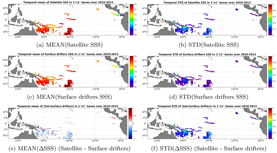
Figure 5: Temporal mean (left) and STD (right) of SSS from SMOS-L3-CATDS-CPDC-V3-10DAYS-25KM (top), Surface drifters (middle), and of \Delta SSS (Satellite - Surface drifters). Only match-up pairs are used to generate these maps.
