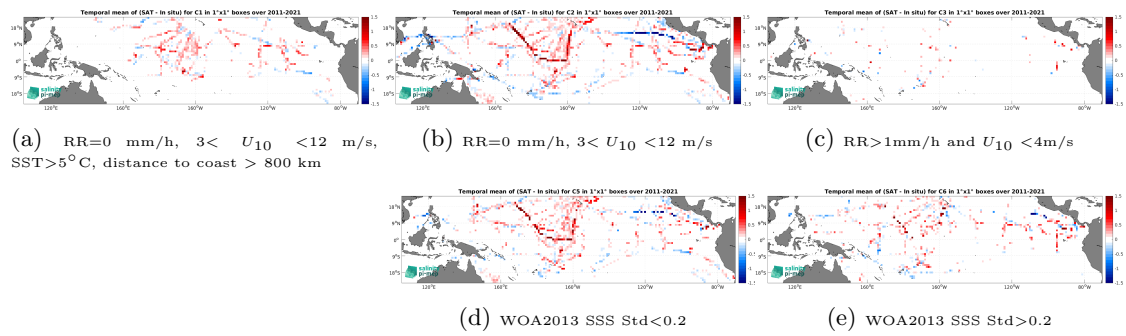
Figure 14: Temporal mean gridded over spatial boxes of size 1^\circ \times 1^\circ of \Delta SSS (SMOS SSS L3 v2 - 9-Days (BEC) - TSG (SAMOS)) for 5 different subdatasets corresponding to:RR=0 mm/h, 3 < U_{10} < 12 m/s, SST >5^\circ\text{C} , distance to coast > 800 km (a), RR=0 mm/h, 3 < U_{10} < 12 m/s (b), RR >1 mm/h and U_{10} < 4 m/s (c), WOA2013 SSS Std <0.2 (d), WOA2013 SSS Std >0.2 (e).
