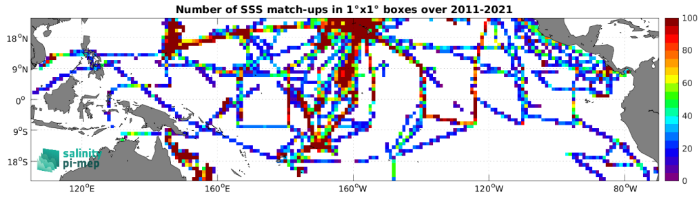
Figure 5: Number of SSS match-ups between TSG (SAMOS) SSS and the SMOS SSS L3 v2 - 9-Days (BEC) SSS product for the Tropical Pacific Ocean Pi-MEP region over 1^\circ \times 1^\circ boxes and for the full satellite product period.
