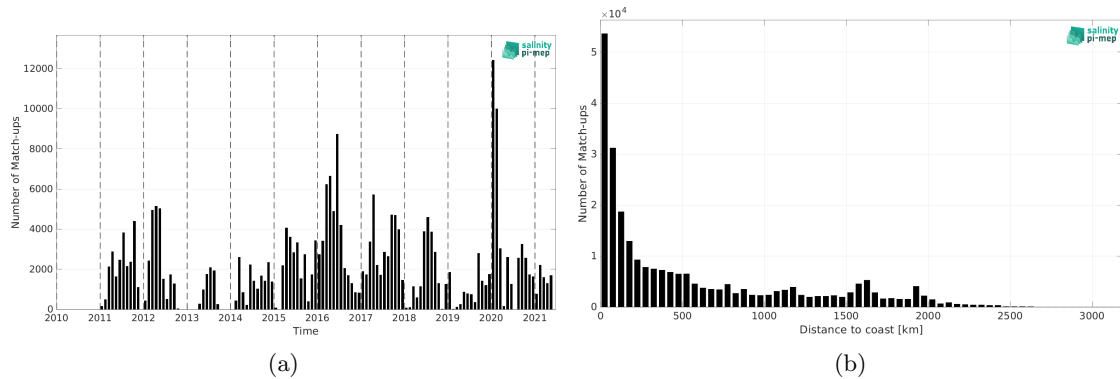
Figure 2: Number of match-ups between TSG (SAMOS) and SMOS SSS L3 v2 - 9-Days (BEC) SSS as a function of time (a) and as function of the distance to coast (b) over the Tropical Pacific Ocean Pi-MEP region and for the full satellite product period.
