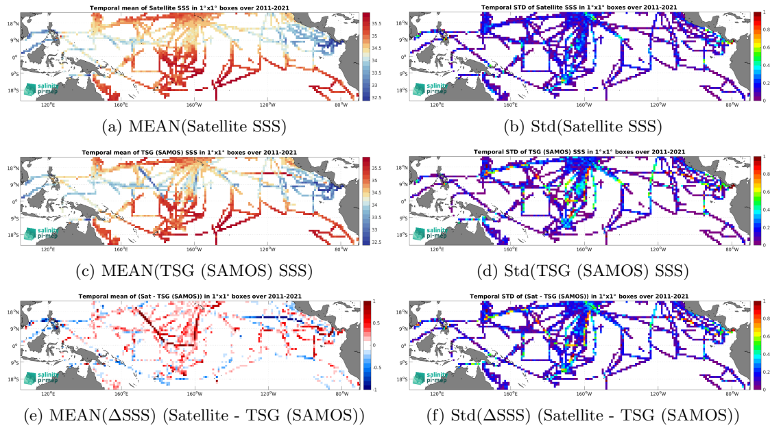
Figure 7: Temporal mean (left) and Std (right) of SSS from SMOS SSS L3 v2 - 9-Days (BEC) (top), TSG (SAMOS) (middle), and of \Delta SSS (Satellite - TSG (SAMOS)). Only match-up pairs are used to generate these maps.
