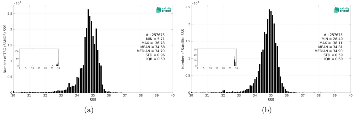
Figure 3: Histograms of SSS from TSG (SAMOS) (a) and SMOS SSS L3 v2 - 9-Days (BEC) (b) considering all match-up pairs per bins of 0.1 over the Tropical Pacific Ocean Pi-MEP region and for the full satellite product period.
