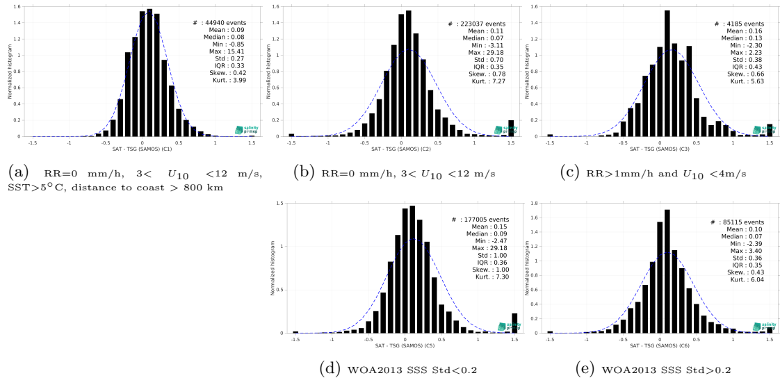
Figure 13: Normalized histogram of \Delta SSS (SMOS SSS L3 v2 - 9-Days (BEC) - TSG (SAMOS)) for 5 different subdatasets corresponding to: RR=0 mm/h, 3 < U_{10} < 12 m/s, SST > 5^\circ\text{C} , distance to coast > 800 km (a), RR=0 mm/h, 3 < U_{10} < 12 m/s (b), RR > 1 mm/h and U_{10} < 4 m/s (c), WOA2013 SSS Std < 0.2 (d), WOA2013 SSS Std > 0.2 (e).
