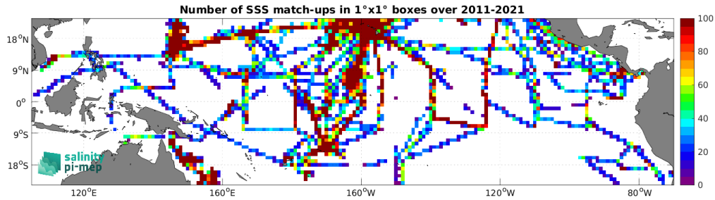
Figure 4: Number of SSS match-ups between TSG (SAMOS) SSS and the SMOS SSS L3 v2 - 9-Days (BEC) SSS product for the Tropical Pacific Ocean Pi-MEP region over 1^\circ \times 1^\circ boxes and for the full satellite product period.
