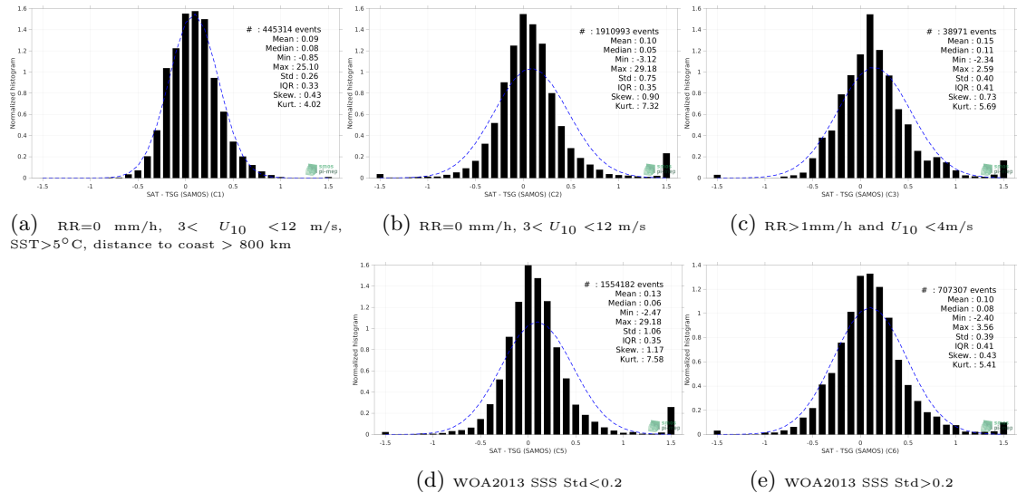
Figure 13: Normalized histogram of \Delta\text{SSS} (SMOS SSS L3 v2 - 9-Days (BEC) - TSG (SAMOS)) for 5 different subdatasets corresponding to: RR=0 mm/h, 3 < U_{10} < 12 m/s, SST >5^\circ\text{C} , distance to coast > 800 km (a), RR=0 mm/h, 3 < U_{10} < 12 m/s (b), RR >1 mm/h and U_{10} < 4 m/s (c), WOA2013 SSS Std <0.2 (d), WOA2013 SSS Std >0.2 (e).
