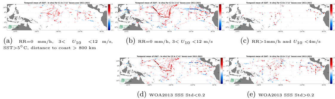
Figure 12: Temporal mean gridded over spatial boxes of size 1^\circ \times 1^\circ of \Delta\text{SSS} (SMOS SSS L3 v2 - 9-Days (BEC) - TSG (SAMOS)) for 5 different subdatasets corresponding to: RR=0 mm/h, 3 < U_{10} < 12 m/s, SST >5^\circ\text{C} , distance to coast > 800 km (a), RR=0 mm/h, 3 < U_{10} < 12 m/s (b), RR >1 mm/h and U_{10} < 4 m/s (c), WOA2013 SSS Std <0.2 (d), WOA2013 SSS Std >0.2 (e).
