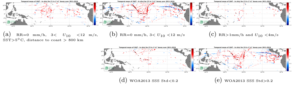
Figure 12: Temporal mean gridded over spatial boxes of size 1^\circ \times 1^\circ of \Delta SSS (SMOS SSS L3 v2 - 9-Days (BEC) - TSG (SAMOS)) for 5 different subdatasets corresponding to: RR=0 mm/h, 3 < U_{10} < 12 m/s, SST > 5^\circ C , distance to coast > 800 km (a), RR=0 mm/h, 3 < U_{10} < 12 m/s (b), RR > 1 mm/h and U_{10} < 4 m/s (c), WOA2013 SSS Std < 0.2 (d), WOA2013 SSS Std > 0.2 (e).
