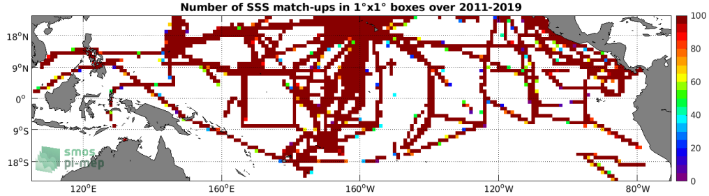
Figure 4: Number of SSS match-ups between TSG (SAMOS) SSS and the SMOS SSS L3 v2 - 9-Days (BEC) SSS product for the Tropical Pacific Ocean Pi-MEP region over 1^\circ \times 1^\circ boxes and for the full satellite product period.
