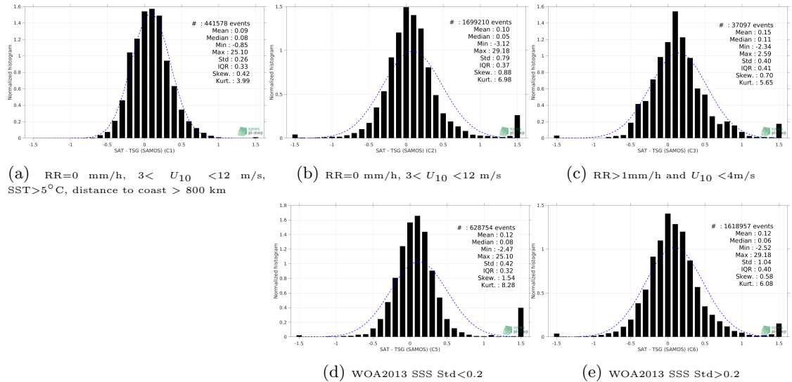
Figure 13: Normalized histogram of \Delta SSS (SMOS SSS L3 v2 - 9-Days (BEC) - TSG (SAMOS)) for 5 different subdatasets corresponding to: RR=0 mm/h, 3 < U_{10} < 12 m/s, SST > 5^\circ C , distance to coast > 800 km (a), RR=0 mm/h, 3 < U_{10} < 12 m/s (b), RR > 1 mm/h and U_{10} < 4 m/s (c), WOA2013 SSS Std < 0.2 (d), WOA2013 SSS Std > 0.2 (e).
