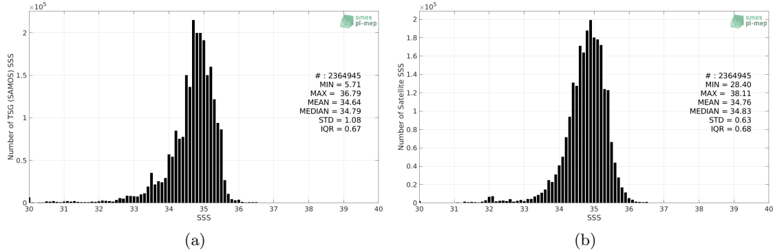
Figure 2: Histograms of SSS from TSG (SAMOS) (a) and SMOS SSS L3 v2 - 9-Days (BEC) (b) considering all match-up pairs per bins of 0.1 over the Tropical Pacific Ocean Pi-MEP region and for the full satellite product period.
