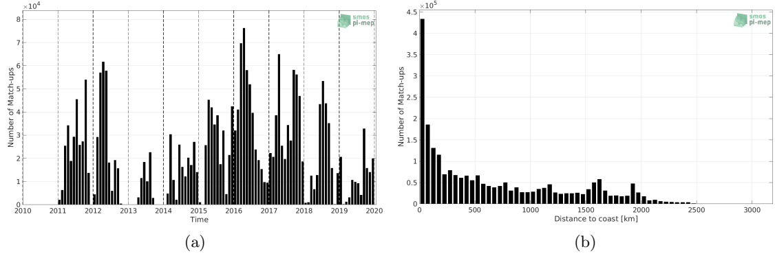
Figure 1: Number of match-ups between TSG (SAMOS) and SMOS SSS L3 v2 - 9-Days (BEC) SSS as a function of time (a) and as function of the distance to coast (b) over the Tropical Pacific Ocean Pi-MEP region and for the full satellite product period.
