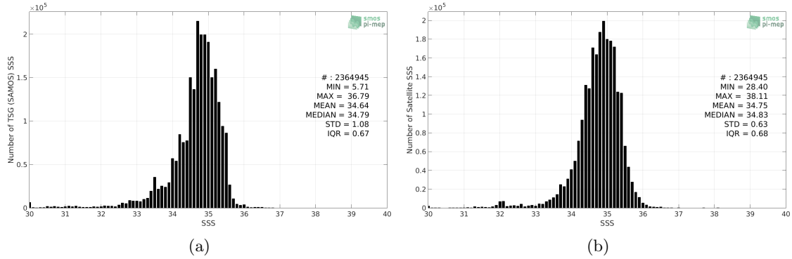
Figure 2: Histograms of SSS from TSG (SAMOS) (a) and SMOS L3 v2 - 9-Days (BEC) (b) considering all match-up pairs per bins of 0.1 over the Tropical Pacific Ocean Pi-MEP region and for the full satellite product period.
