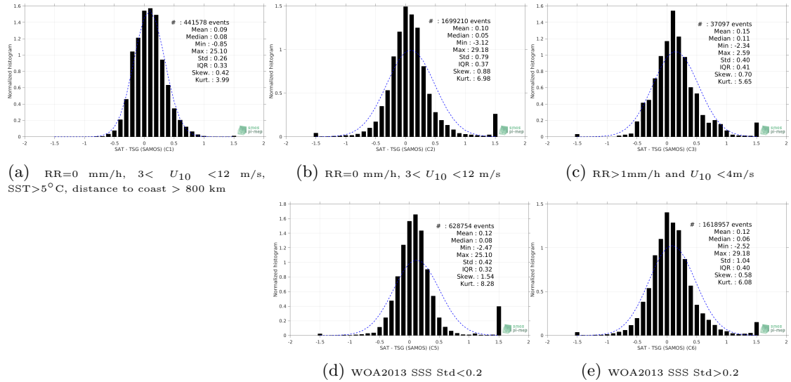
Figure 13: Normalized histogram of \Delta SSS (SMOS L3 v2 - 9-Days (BEC) - TSG (SAMOS)) for 5 different subdatasets corresponding to: RR=0 mm/h, 3 < U_{10} < 12 m/s, SST > 5^\circ C , distance to coast > 800 km (a), RR=0 mm/h, 3 < U_{10} < 12 m/s (b), RR > 1 mm/h and U_{10} < 4 m/s (c), WOA2013 SSS Std < 0.2 (d), WOA2013 SSS Std > 0.2 (e).
