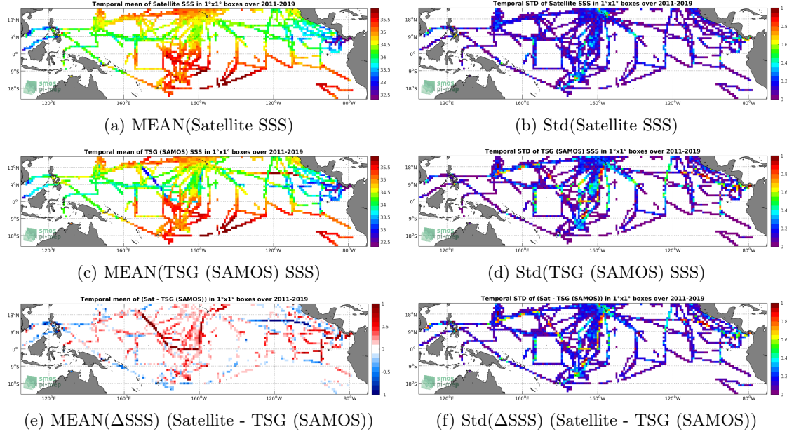
Figure 6: Temporal mean (left) and Std (right) of SSS from SMOS L3 v2 - 9-Days (BEC) (top), TSG (SAMOS) (middle), and of \Delta SSS (Satellite - TSG (SAMOS)). Only match-up pairs are used to generate these maps.
