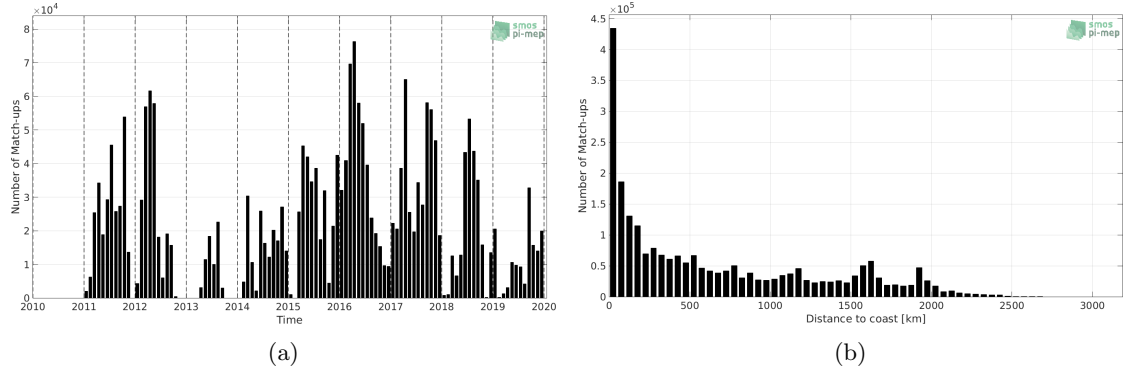
Figure 1: Number of match-ups between TSG (SAMOS) and SMOS L3 v2 - 9-Days (BEC) SSS as a function of time (a) and as function of the distance to coast (b) over the Tropical Pacific Ocean Pi-MEP region and for the full satellite product period.
