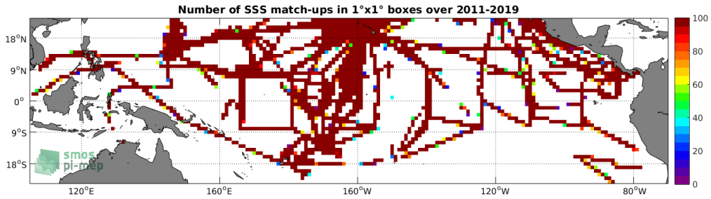
Figure 4: Number of SSS match-ups between TSG (SAMOS) SSS and the SMOS L3 v2 - 9-Days (BEC) SSS product for the Tropical Pacific Ocean Pi-MEP region over 1°x1° boxes and for the full satellite product period.
