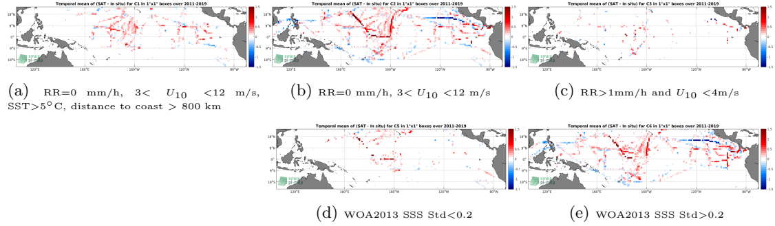
Figure 12: Temporal mean gridded over spatial boxes of size 1^\circ \times 1^\circ of \Delta SSS (SMOS L3 v2 - 9-Days (BEC) - TSG (SAMOS)) for 5 different subdatasets corresponding to: RR=0 mm/h, 3 < U_{10} < 12 m/s, SST > 5^\circ C , distance to coast > 800 km (a), RR=0 mm/h, 3 < U_{10} < 12 m/s (b), RR > 1 mm/h and U_{10} < 4 m/s (c), WOA2013 SSS Std < 0.2 (d), WOA2013 SSS Std > 0.2 (e).
