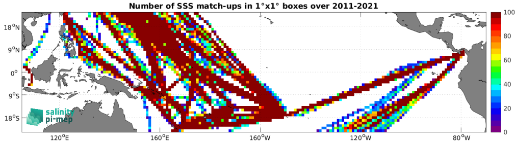
Figure 5: Number of SSS match-ups between TSG (LEGOS-DM) SSS and the SMOS SSS L3 v2 - 9-Days (BEC) SSS product for the Tropical Pacific Ocean Pi-MEP region over 1^\circ \times 1^\circ boxes and for the full satellite product period.
