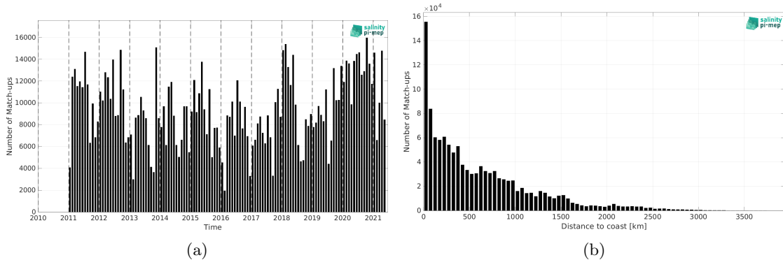
Figure 2: Number of match-ups between TSG (LEGOS-DM) and SMOS SSS L3 v2 - 9-Days (BEC) SSS as a function of time (a) and as function of the distance to coast (b) over the Tropical Pacific Ocean Pi-MEP region and for the full satellite product period.
