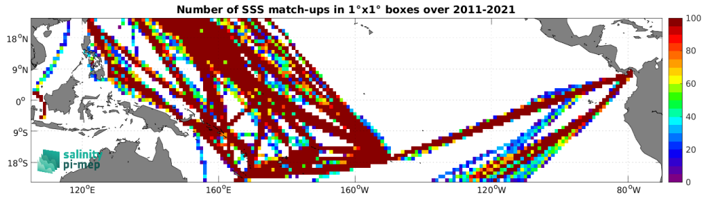
Figure 5: Number of SSS match-ups between TSG (LEGOS-DM) SSS and the SMOS SSS L3 v2 - 9-Days (BEC) SSS product for the Tropical Pacific Ocean Pi-MEP region over 1^\circ \times 1^\circ boxes and for the full satellite product period.
