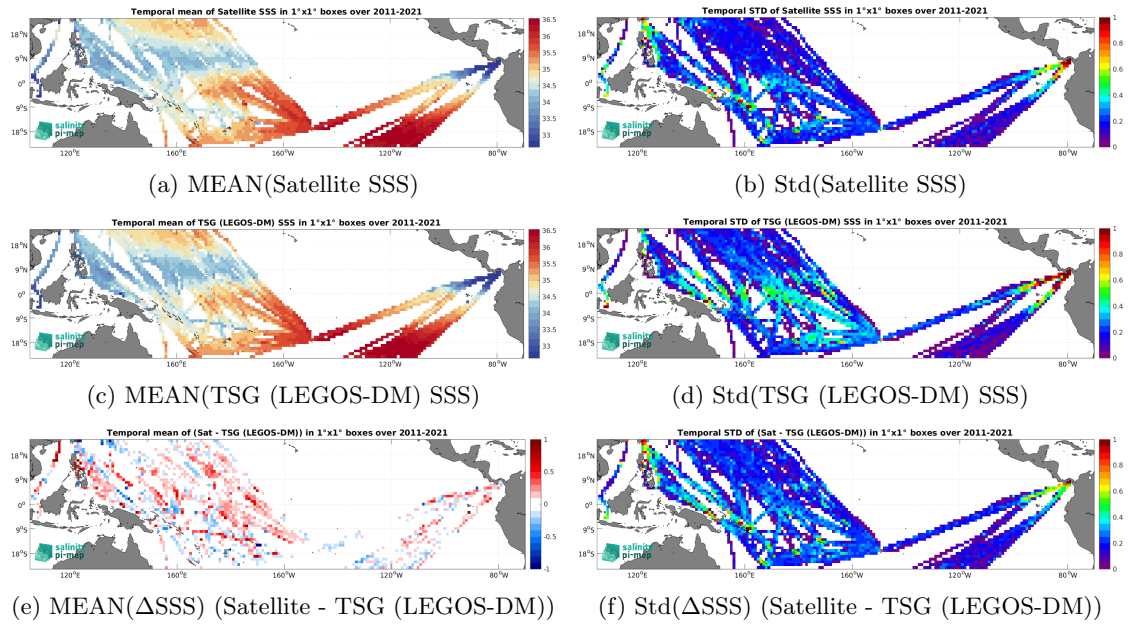
Figure 7: Temporal mean (left) and Std (right) of SSS from SMOS SSS L3 v2 - 9-Days (BEC) (top), TSG (LEGOS-DM) (middle), and of \Delta SSS (Satellite - TSG (LEGOS-DM)). Only match-up pairs are used to generate these maps.
