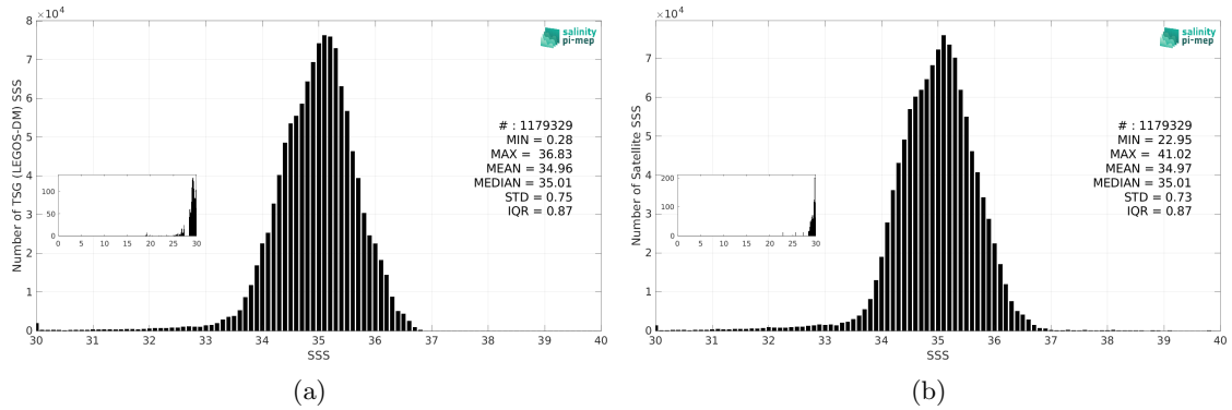
Figure 3: Histograms of SSS from TSG (LEGOS-DM) (a) and SMOS SSS L3 v2 - 9-Days (BEC) (b) considering all match-up pairs per bins of 0.1 over the Tropical Pacific Ocean Pi-MEP region and for the full satellite product period.
