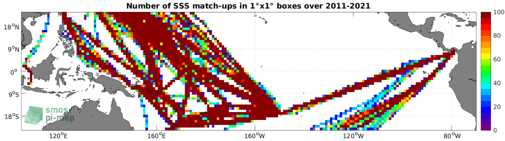
Figure 4: Number of SSS match-ups between TSG (LEGOS-DM) SSS and the SMOS SSS L3 v2 - 9-Days (BEC) SSS product for the Tropical Pacific Ocean Pi-MEP region over 1^\circ \times 1^\circ boxes and for the full satellite product period.
