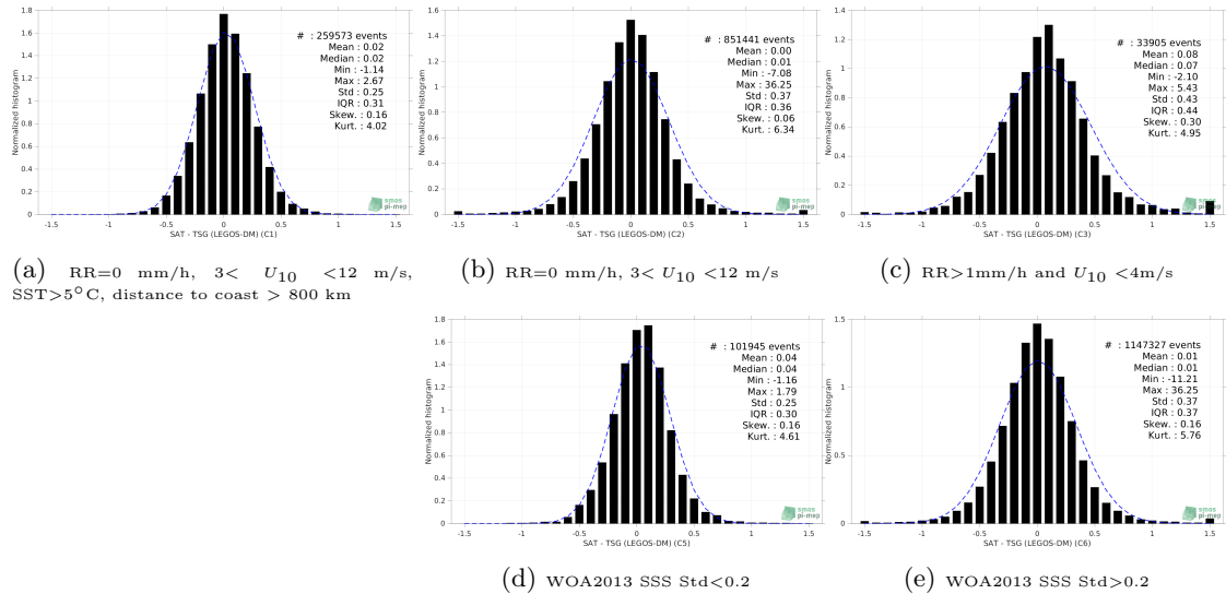
Figure 13: Normalized histogram of \Delta SSS (SMOS SSS L3 v2 - 9-Days (BEC) - TSG (LEGOS-DM)) for 5 different subdatasets corresponding to: RR=0 mm/h, 3 < U_{10} < 12 m/s, SST >5^\circ C, distance to coast > 800 km (a), RR=0 mm/h, 3 < U_{10} < 12 m/s (b), RR >1 mm/h and U_{10} < 4 m/s (c), WOA2013 SSS Std <0.2 (d), WOA2013 SSS Std >0.2 (e).
