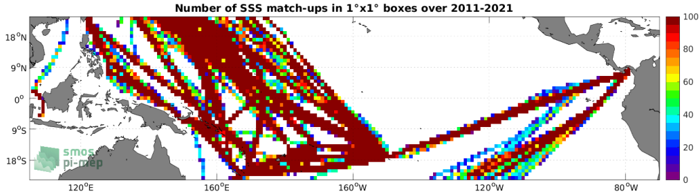
Figure 4: Number of SSS match-ups between TSG (LEGOS-DM) SSS and the SMOS SSS L3 v2 - 9-Days (BEC) SSS product for the Tropical Pacific Ocean Pi-MEP region over 1^\circ \times 1^\circ boxes and for the full satellite product period.
