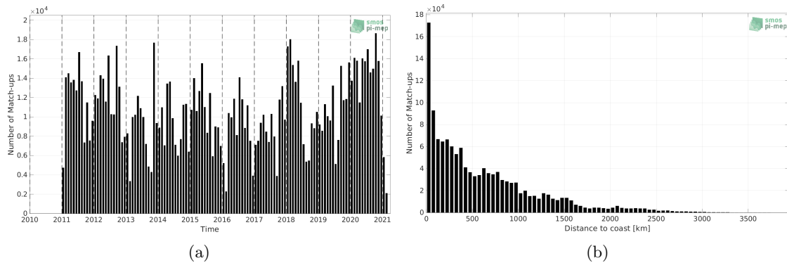
Figure 1: Number of match-ups between TSG (LEGOS-DM) and SMOS SSS L3 v2 - 9-Days (BEC) SSS as a function of time (a) and as function of the distance to coast (b) over the Tropical Pacific Ocean Pi-MEP region and for the full satellite product period.
