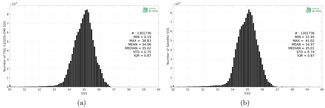
Figure 2: Histograms of SSS from TSG (LEGOS-DM) (a) and SMOS SSS L3 v2 - 9-Days (BEC) (b) considering all match-up pairs per bins of 0.1 over the Tropical Pacific Ocean Pi-MEP region and for the full satellite product period.
