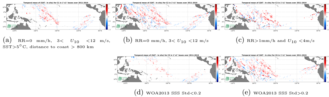
Figure 12: Temporal mean gridded over spatial boxes of size 1°x1° of ΔSSS (SMOS SSS L3 v2 - 9-Days (BEC) - TSG (LEGOS-DM)) for 5 different subdatasets corresponding to:RR=0 mm/h, 3 < U_{10} < 12 m/s, SST>5°C, distance to coast > 800 km (a), RR=0 mm/h, 3 < U_{10} < 12 m/s (b), RR>1mm/h and U_{10} < 4m/s (c), WOA2013 SSS Std<0.2 (d), WOA2013 SSS Std>0.2 (e).
