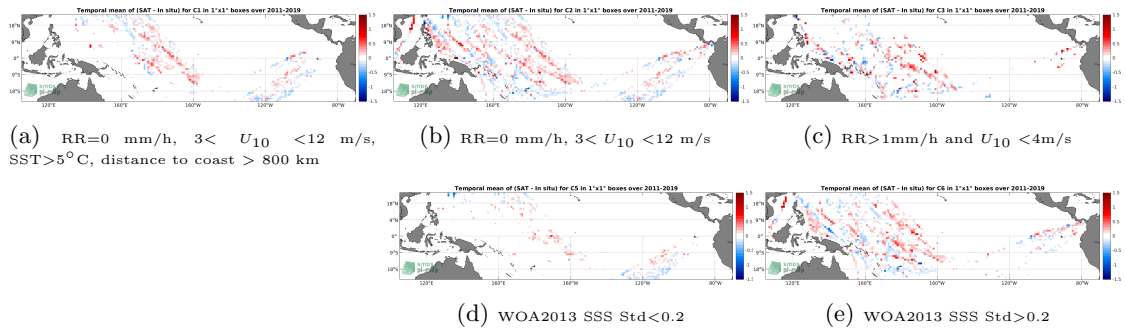
Figure 12: Temporal mean gridded over spatial boxes of size 1°x1° of ΔSSS (SMOS SSS L3 v2 - 9-Days (BEC) - TSG (LEGOS-DM)) for 5 different subdatasets corresponding to:RR=0 mm/h, 3 < U_{10} < 12 m/s, SST>5°C, distance to coast > 800 km (a), RR=0 mm/h, 3 < U_{10} < 12 m/s (b), RR>1mm/h and U_{10} < 4m/s (c), WOA2013 SSS Std<0.2 (d), WOA2013 SSS Std>0.2 (e).
