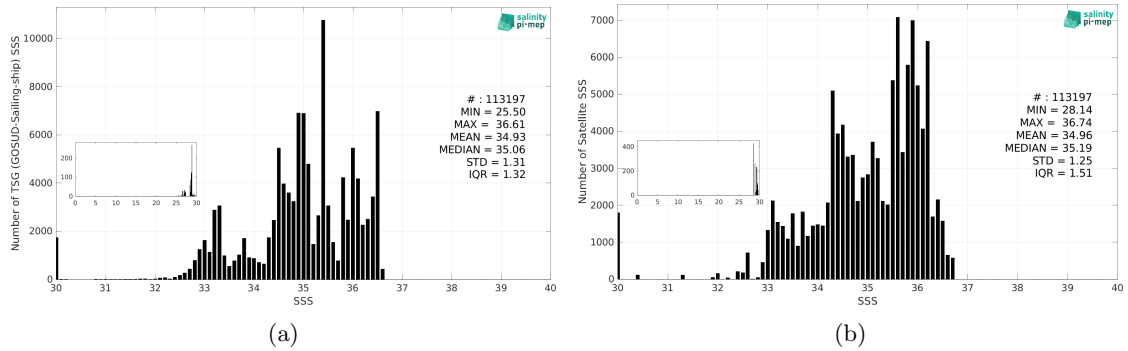
Figure 3: Histograms of SSS from TSG (GOSUD-Sailing-ship) (a) and SMOS SSS L3 v2 - 9-Days (BEC) (b) considering all match-up pairs per bins of 0.1 over the Tropical Pacific Ocean Pi-MEP region and for the full satellite product period.
