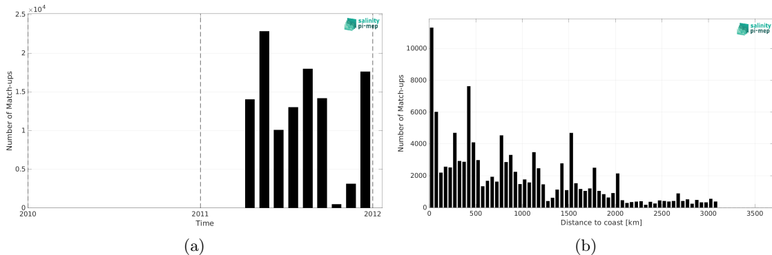
Figure 2: Number of match-ups between TSG (GOSUD-Sailing-ship) and SMOS SSS L3 v2 - 9-Days (BEC) SSS as a function of time (a) and as function of the distance to coast (b) over the Tropical Pacific Ocean Pi-MEP region and for the full satellite product period.
