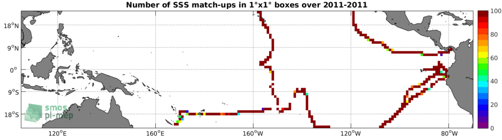
Figure 4: Number of SSS match-ups between TSG (GOSUD-Sailing-ship) SSS and the SMOS SSS L3 v2 - 9-Days (BEC) SSS product for the Tropical Pacific Ocean Pi-MEP region over 1^\circ \times 1^\circ boxes and for the full satellite product period.
