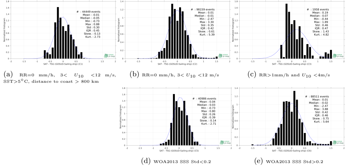
Figure 13: Normalized histogram of \Delta SSS (SMOS SSS L3 v2 - 9-Days (BEC) - TSG (GOSUD-Sailing-ship)) for 5 different subdatasets corresponding to: RR=0 mm/h, 3 < U_{10} < 12 m/s, SST>5°C, distance to coast > 800 km (a), RR=0 mm/h, 3 < U_{10} < 12 m/s (b), RR>1mm/h and U_{10} < 4 m/s (c), WOA2013 SSS Std<0.2 (d), WOA2013 SSS Std>0.2 (e).
