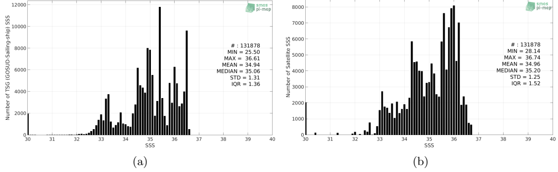
Figure 2: Histograms of SSS from TSG (GOSUD-Sailing-ship) (a) and SMOS SSS L3 v2 - 9-Days (BEC) (b) considering all match-up pairs per bins of 0.1 over the Tropical Pacific Ocean Pi-MEP region and for the full satellite product period.
