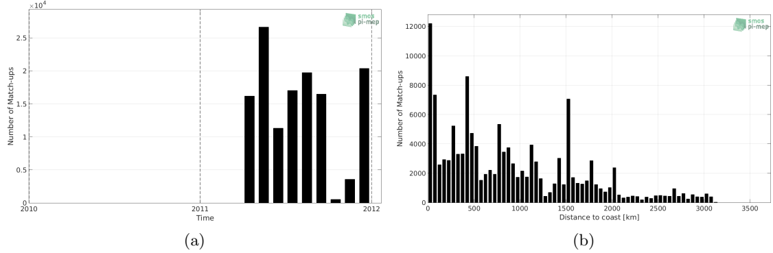
Figure 1: Number of match-ups between TSG (GOSUD-Sailing-ship) and SMOS SSS L3 v2 - 9-Days (BEC) SSS as a function of time (a) and as function of the distance to coast (b) over the Tropical Pacific Ocean Pi-MEP region and for the full satellite product period.
