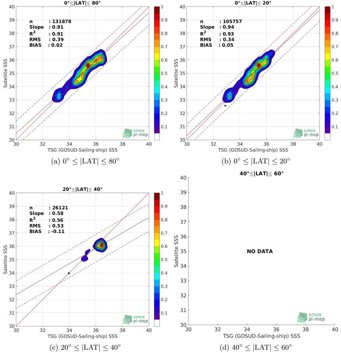
Figure 9: Contour maps of the concentration of SMOS L3 v2 - 9-Days (BEC) SSS (y-axis) versus TSG (GOSUD-Sailing-ship) SSS (x-axis) at match-up pairs for different latitude bands. For each plot, the red line shows x=y . The black thin and dashed lines indicate a linear fit through the data cloud and the \pm 95\% confidence levels, respectively. The number match-up pairs n , the slope and R^2 coefficient of the linear fit, the root mean square (RMS) and the mean bias between satellite and in situ data are indicated for each latitude band in each plots.
