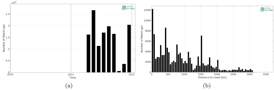
Figure 1: Number of match-ups between TSG (GOSUD-Sailing-ship) and SMOS L3 v2 - 9-Days (BEC) SSS as a function of time (a) and as function of the distance to coast (b) over the Tropical Pacific Ocean Pi-MEP region and for the full satellite product period.
