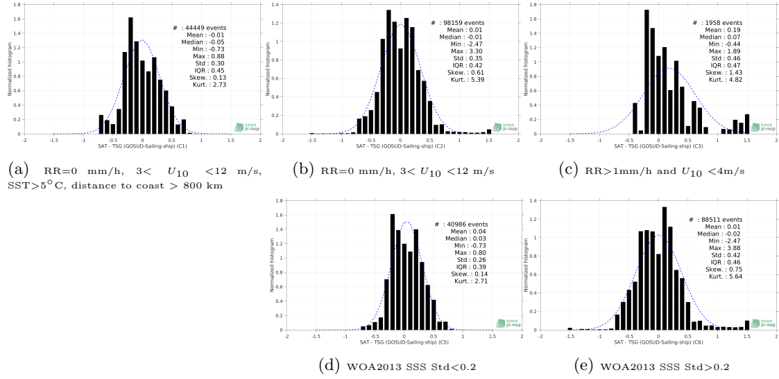
Figure 13: Normalized histogram of \Delta SSS (SMOS L3 v2 - 9-Days (BEC) - TSG (GOSUD-Sailing-ship)) for 5 different subdatasets corresponding to: RR=0 mm/h, 3 < U_{10} < 12 m/s, SST>5°C, distance to coast > 800 km (a), RR=0 mm/h, 3 < U_{10} < 12 m/s (b), RR>1mm/h and U_{10} < 4 m/s (c), WOA2013 SSS Std<0.2 (d), WOA2013 SSS Std>0.2 (e).
