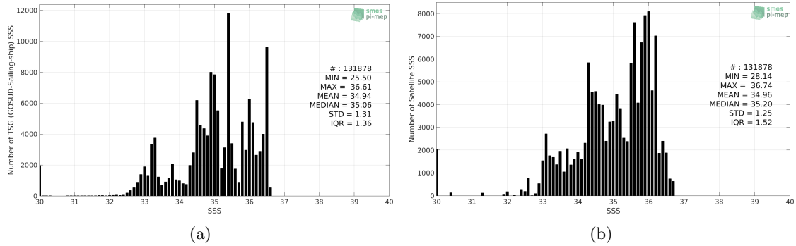
Figure 2: Histograms of SSS from TSG (GOSUD-Sailing-ship) (a) and SMOS L3 v2 - 9-Days (BEC) (b) considering all match-up pairs per bins of 0.1 over the Tropical Pacific Ocean Pi-MEP region and for the full satellite product period.
