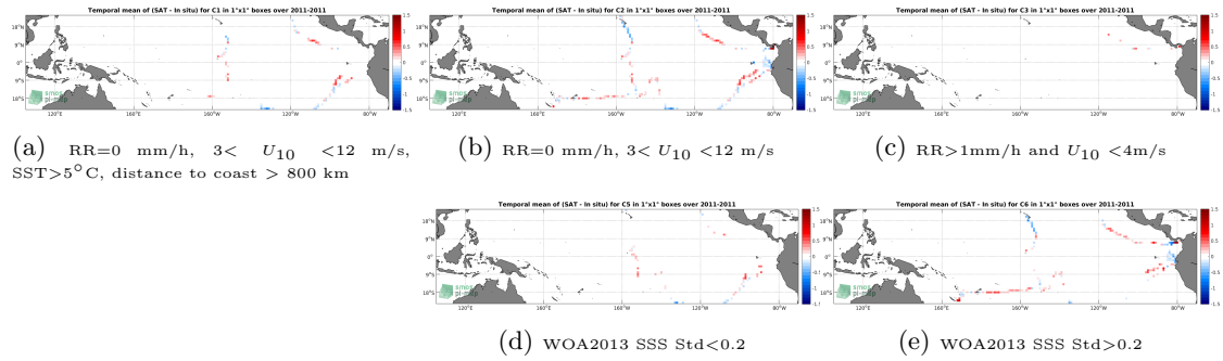
Figure 12: Temporal mean gridded over spatial boxes of size 1^\circ \times 1^\circ of \Delta SSS (SMOS L3 v2 - 9-Days (BEC) - TSG (GOSUD-Sailing-ship)) for 5 different subdatasets corresponding to: RR=0 mm/h, 3 < U_{10} < 12 m/s, SST > 5^\circ\text{C} , distance to coast > 800 km (a), RR=0 mm/h, 3 < U_{10} < 12 m/s (b), RR > 1\text{mm/h} and U_{10} < 4\text{m/s} (c), WOA2013 SSS Std < 0.2 (d), WOA2013 SSS Std > 0.2 (e).
