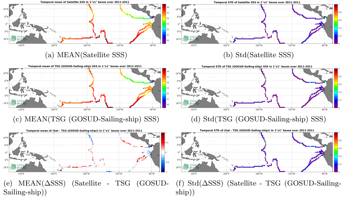
Figure 6: Temporal mean (left) and Std (right) of SSS from SMOS L3 v2 - 9-Days (BEC) (top), TSG (GOSUD-Sailing-ship) (middle), and of \Delta SSS (Satellite - TSG (GOSUD-Sailing-ship)). Only match-up pairs are used to generate these maps.
