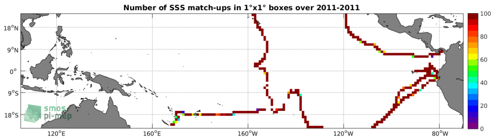
Figure 4: Number of SSS match-ups between TSG (GOSUD-Sailing-ship) SSS and the SMOS L3 v2 - 9-Days (BEC) SSS product for the Tropical Pacific Ocean Pi-MEP region over 1^\circ \times 1^\circ boxes and for the full satellite product period.
