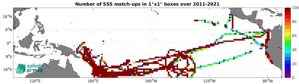
Figure 5: Number of SSS match-ups between TSG (GOSUD-Research-vessel) SSS and the SMOS SSS L3 v2 - 9-Days (BEC) SSS product for the Tropical Pacific Ocean Pi-MEP region over 1^\circ \times 1^\circ boxes and for the full satellite product period.
