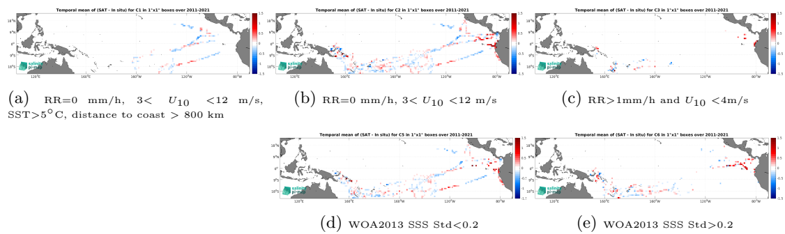
Figure 14: Temporal mean gridded over spatial boxes of size 1^\circ \times 1^\circ of \Delta SSS (SMOS SSS L3 v2 - 9-Days (BEC) - TSG (GOSUD-Research-vessel)) for 5 different subdatasets corresponding to: RR=0 mm/h, 3 < U_{10} < 12 m/s, SST > 5^\circ\text{C} , distance to coast > 800 km (a), RR=0 mm/h, 3 < U_{10} < 12 m/s (b), RR > 1 mm/h and U_{10} < 4 m/s (c), WOA2013 SSS Std < 0.2 (d), WOA2013 SSS Std > 0.2 (e).
