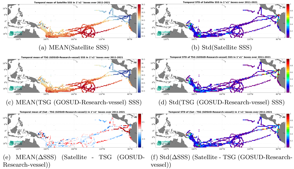
Figure 7: Temporal mean (left) and Std (right) of SSS from SMOS SSS L3 v2 - 9-Days (BEC) (top), TSG (GOSUD-Research-vessel) (middle), and of \Delta SSS (Satellite - TSG (GOSUD-Research-vessel)). Only match-up pairs are used to generate these maps.
