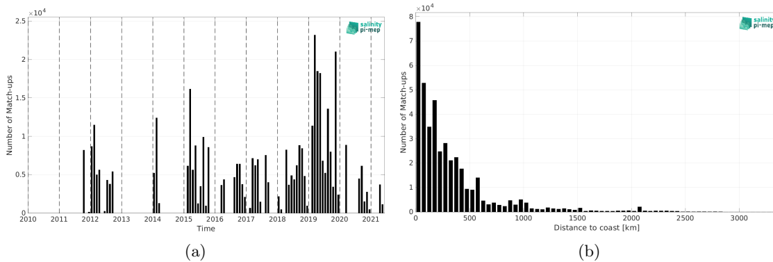
Figure 2: Number of match-ups between TSG (GOSUD-Research-vessel) and SMOS SSS L3 v2 - 9-Days (BEC) SSS as a function of time (a) and as function of the distance to coast (b) over the Tropical Pacific Ocean Pi-MEP region and for the full satellite product period.
