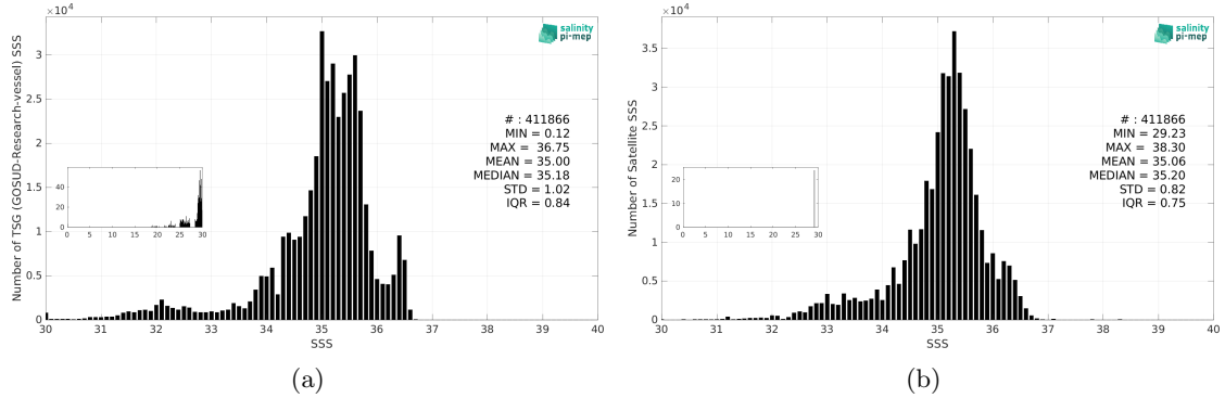
Figure 3: Histograms of SSS from TSG (GOSUD-Research-vessel) (a) and SMOS SSS L3 v2 - 9-Days (BEC) (b) considering all match-up pairs per bins of 0.1 over the Tropical Pacific Ocean Pi-MEP region and for the full satellite product period.
