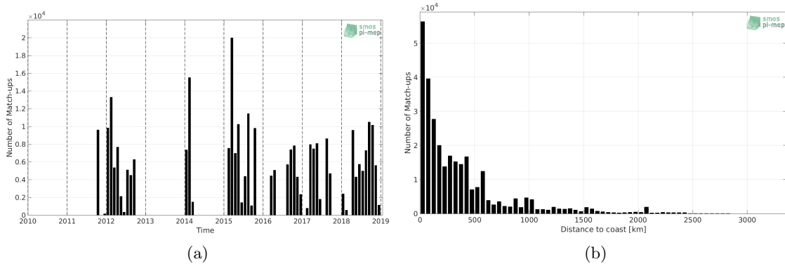
Figure 1: Number of match-ups between TSG (GOSUD-Research-vessel) and SMOS L3 v2 - 9-Days (BEC) SSS as a function of time (a) and as function of the distance to coast (b) over the Tropical Pacific Ocean Pi-MEP region and for the full satellite product period.
