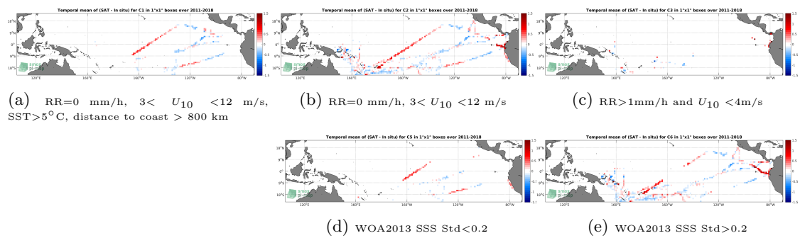
Figure 12: Temporal mean gridded over spatial boxes of size 1^\circ \times 1^\circ of \Delta SSS (SMOS L3 v2 - 9-Days (BEC) - TSG (GOSUD-Research-vessel)) for 5 different subdatasets corresponding to:RR=0 mm/h, 3 < U_{10} < 12 m/s, SST>5°C, distance to coast > 800 km (a), RR=0 mm/h, 3 < U_{10} < 12 m/s (b), RR>1mm/h and U_{10} < 4 m/s (c), WOA2013 SSS Std<0.2 (d), WOA2013 SSS Std>0.2 (e).
