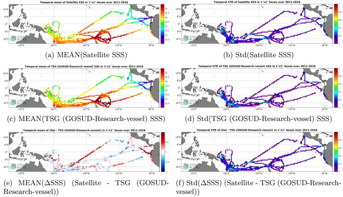
Figure 6: Temporal mean (left) and Std (right) of SSS from SMOS L3 v2 - 9-Days (BEC) (top), TSG (GOSUD-Research-vessel) (middle), and of \Delta SSS (Satellite - TSG (GOSUD-Research-vessel)). Only match-up pairs are used to generate these maps.
