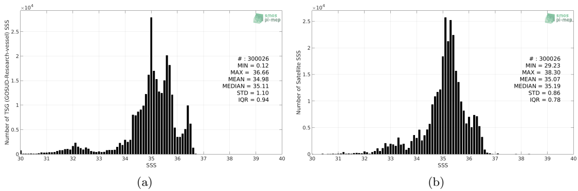
Figure 2: Histograms of SSS from TSG (GOSUD-Research-vessel) (a) and SMOS L3 v2 - 9-Days (BEC) (b) considering all match-up pairs per bins of 0.1 over the Tropical Pacific Ocean Pi-MEP region and for the full satellite product period.
