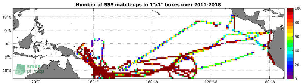
Figure 4: Number of SSS match-ups between TSG (GOSUD-Research-vessel) SSS and the SMOS L3 v2 - 9-Days (BEC) SSS product for the Tropical Pacific Ocean Pi-MEP region over 1^\circ \times 1^\circ boxes and for the full satellite product period.
