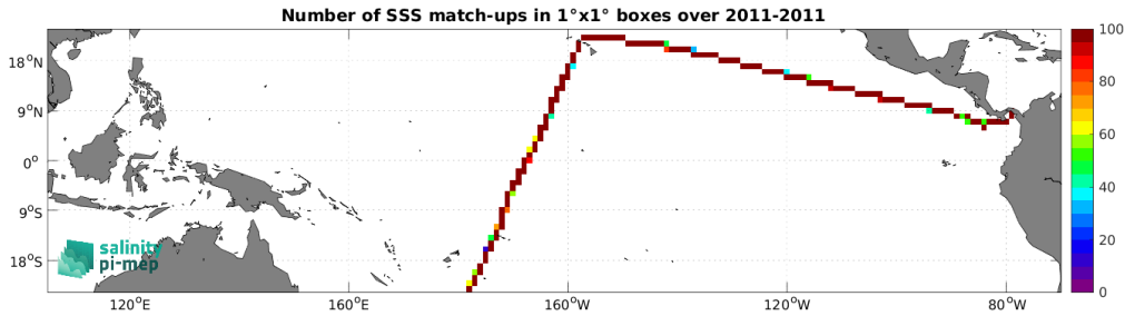
Figure 5: Number of SSS match-ups between TSG (CSIC-UTM) SSS and the SMOS SSS L3 v2 - 9-Days (BEC) SSS product for the Tropical Pacific Ocean Pi-MEP region over 1^\circ \times 1^\circ boxes and for the full satellite product period.
