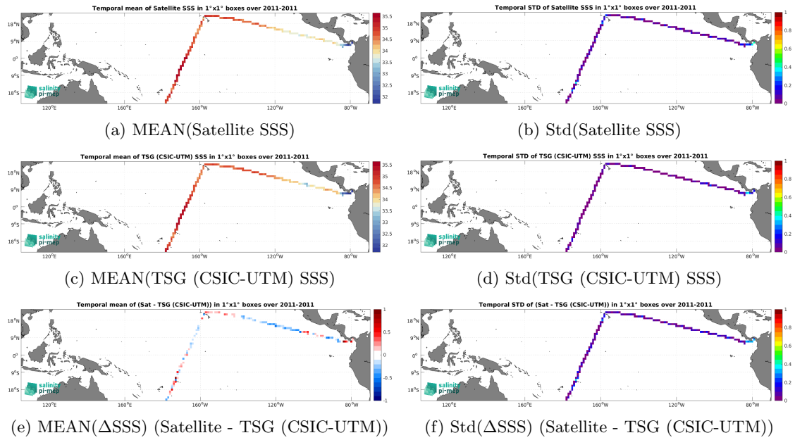
Figure 7: Temporal mean (left) and Std (right) of SSS from SMOS SSS L3 v2 - 9-Days (BEC) (top), TSG (CSIC-UTM) (middle), and of \Delta SSS (Satellite - TSG (CSIC-UTM)). Only match-up pairs are used to generate these maps.
