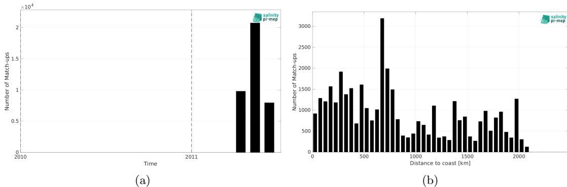
Figure 2: Number of match-ups between TSG (CSIC-UTM) and SMOS SSS L3 v2 - 9-Days (BEC) SSS as a function of time (a) and as function of the distance to coast (b) over the Tropical Pacific Ocean Pi-MEP region and for the full satellite product period.
