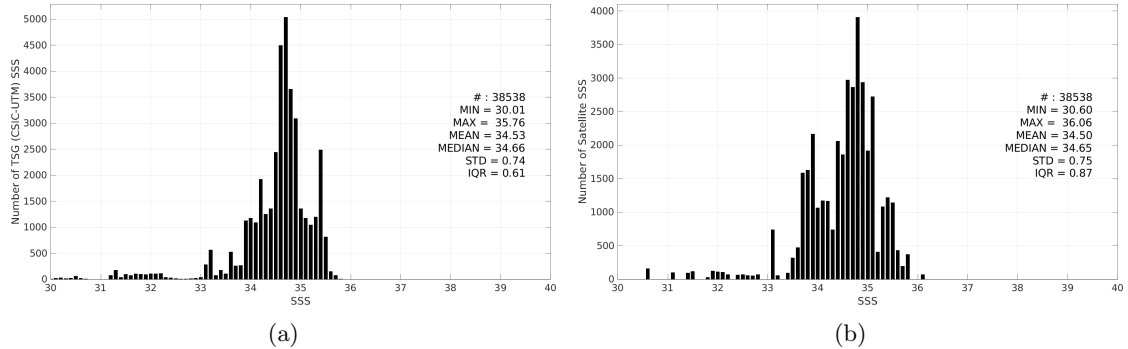
Figure 3: Histograms of SSS from TSG (CSIC-UTM) (a) and SMOS SSS L3 v2 - 9-Days (BEC) (b) considering all match-up pairs per bins of 0.1 over the Tropical Pacific Ocean Pi-MEP region and for the full satellite product period.
