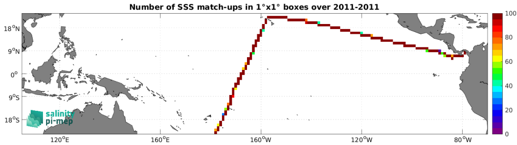
Figure 4: Number of SSS match-ups between TSG (CSIC-UTM) SSS and the SMOS SSS L3 v2 - 9-Days (BEC) SSS product for the Tropical Pacific Ocean Pi-MEP region over 1^\circ \times 1^\circ boxes and for the full satellite product period.
