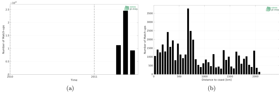
Figure 1: Number of match-ups between TSG (CSIC-UTM) and SMOS SSS L3 v2 - 9-Days (BEC) SSS as a function of time (a) and as function of the distance to coast (b) over the Tropical Pacific Ocean Pi-MEP region and for the full satellite product period.
