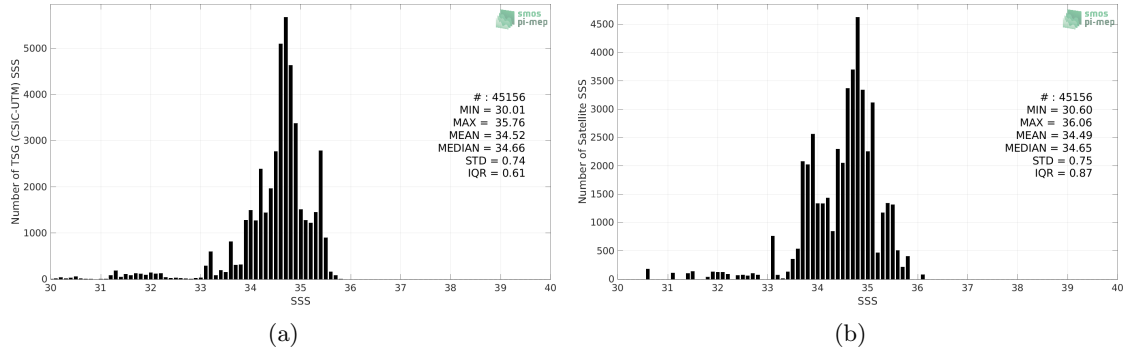
Figure 2: Histograms of SSS from TSG (CSIC-UTM) (a) and SMOS SSS L3 v2 - 9-Days (BEC) (b) considering all match-up pairs per bins of 0.1 over the Tropical Pacific Ocean Pi-MEP region and for the full satellite product period.
