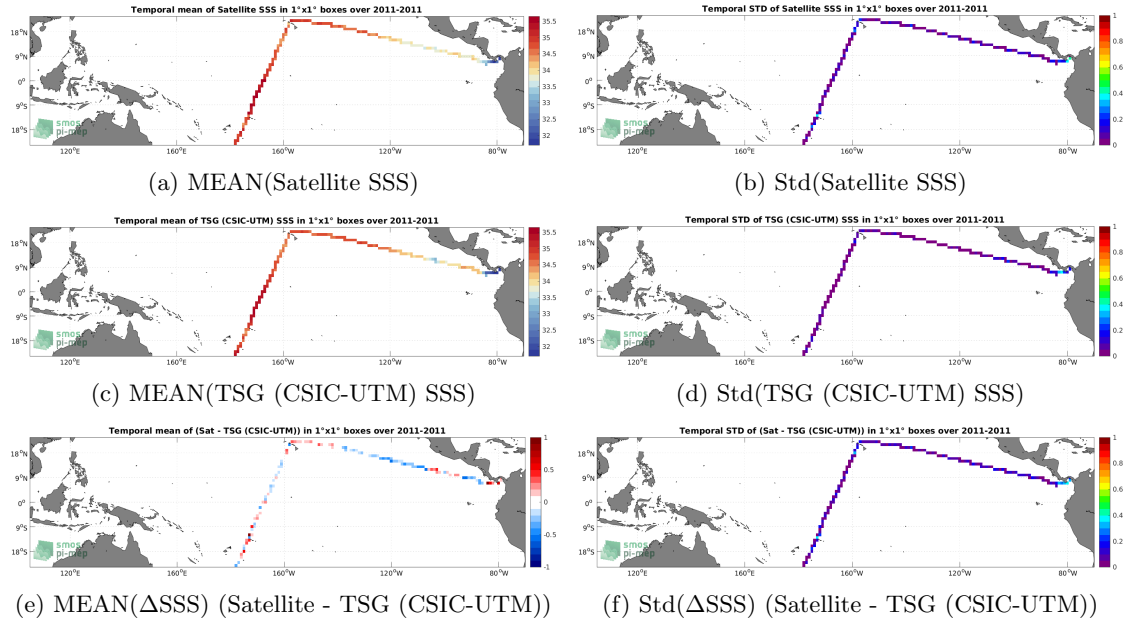
Figure 6: Temporal mean (left) and Std (right) of SSS from SMOS SSS L3 v2 - 9-Days (BEC) (top), TSG (CSIC-UTM) (middle), and of \Delta SSS (Satellite - TSG (CSIC-UTM)). Only match-up pairs are used to generate these maps.
