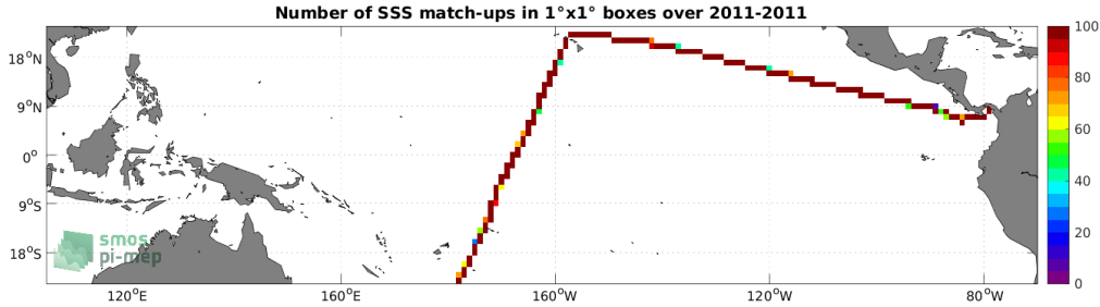
Figure 4: Number of SSS match-ups between TSG (CSIC-UTM) SSS and the SMOS SSS L3 v2 - 9-Days (BEC) SSS product for the Tropical Pacific Ocean Pi-MEP region over 1^\circ \times 1^\circ boxes and for the full satellite product period.
