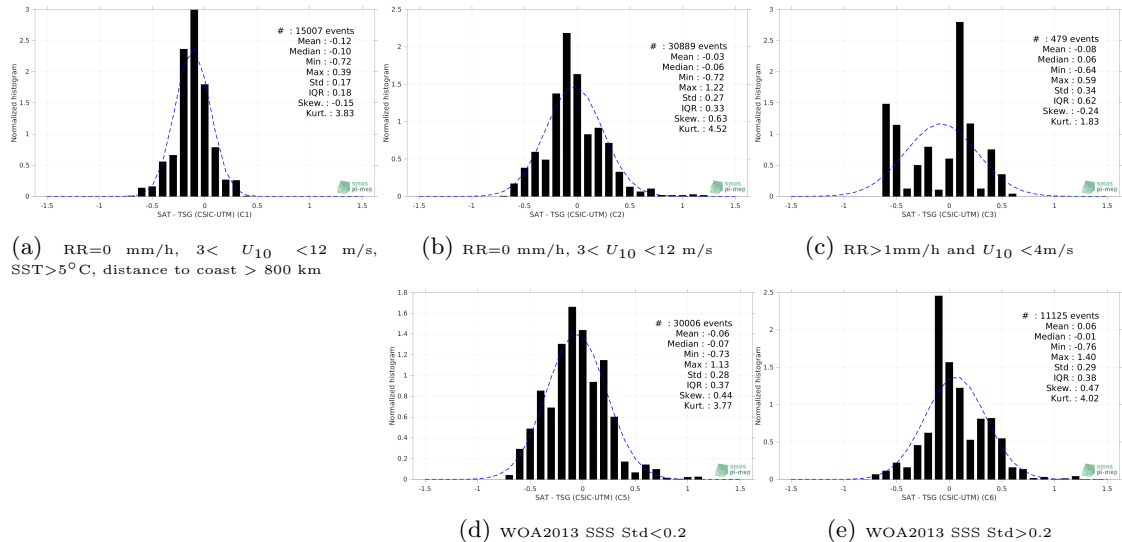
Figure 13: Normalized histogram of \Delta SSS (SMOS SSS L3 v2 - 9-Days (BEC) - TSG (CSIC-UTM)) for 5 different subdatasets corresponding to: RR=0 mm/h, 3 < U_{10} < 12 m/s, SST >5^\circ C, distance to coast > 800 km (a), RR=0 mm/h, 3 < U_{10} < 12 m/s (b), RR >1 mm/h and U_{10} < 4 m/s (c), WOA2013 SSS Std <0.2 (d), WOA2013 SSS Std >0.2 (e).
