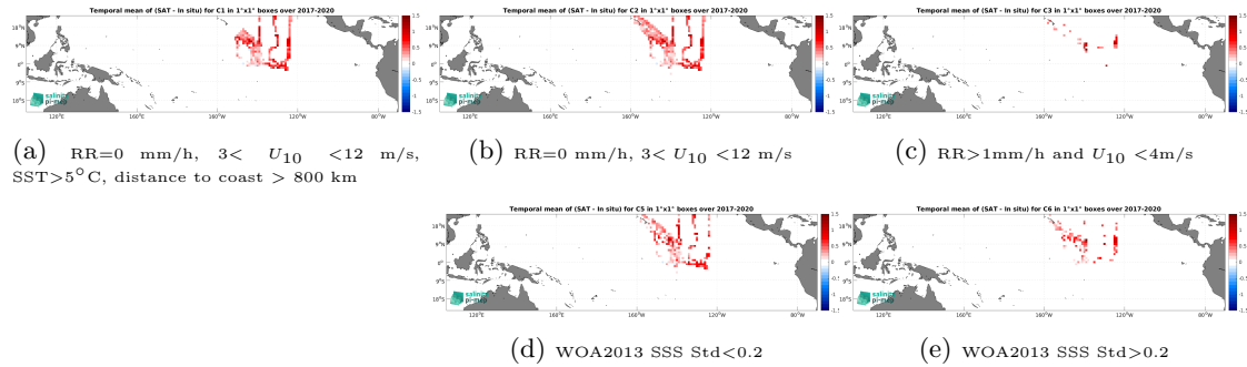
Figure 12: Temporal mean gridded over spatial boxes of size 1^\circ \times 1^\circ of \Delta\text{SSS} (SMOS SSS L3 v2 - 9-Days (BEC) - Saildrone) for 5 different subdatasets corresponding to:RR=0 mm/h, 3 < U_{10} < 12 m/s, SST >5^\circ\text{C} , distance to coast > 800 km (a), RR=0 mm/h, 3 < U_{10} < 12 m/s (b), RR >1 mm/h and U_{10} < 4 m/s (c), WOA2013 SSS Std <0.2 (d), WOA2013 SSS Std >0.2 (e).
