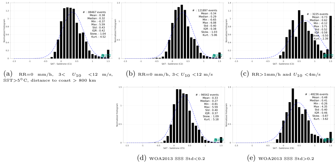
Figure 13: Normalized histogram of \Delta\text{SSS} (SMOS SSS L3 v2 - 9-Days (BEC) - Saildrone) for 5 different subdatasets corresponding to: RR=0 mm/h, 3 < U_{10} < 12 m/s, SST >5^\circ\text{C} , distance to coast > 800 km (a), RR=0 mm/h, 3 < U_{10} < 12 m/s (b), RR >1 mm/h and U_{10} < 4 m/s (c), WOA2013 SSS Std <0.2 (d), WOA2013 SSS Std >0.2 (e).
