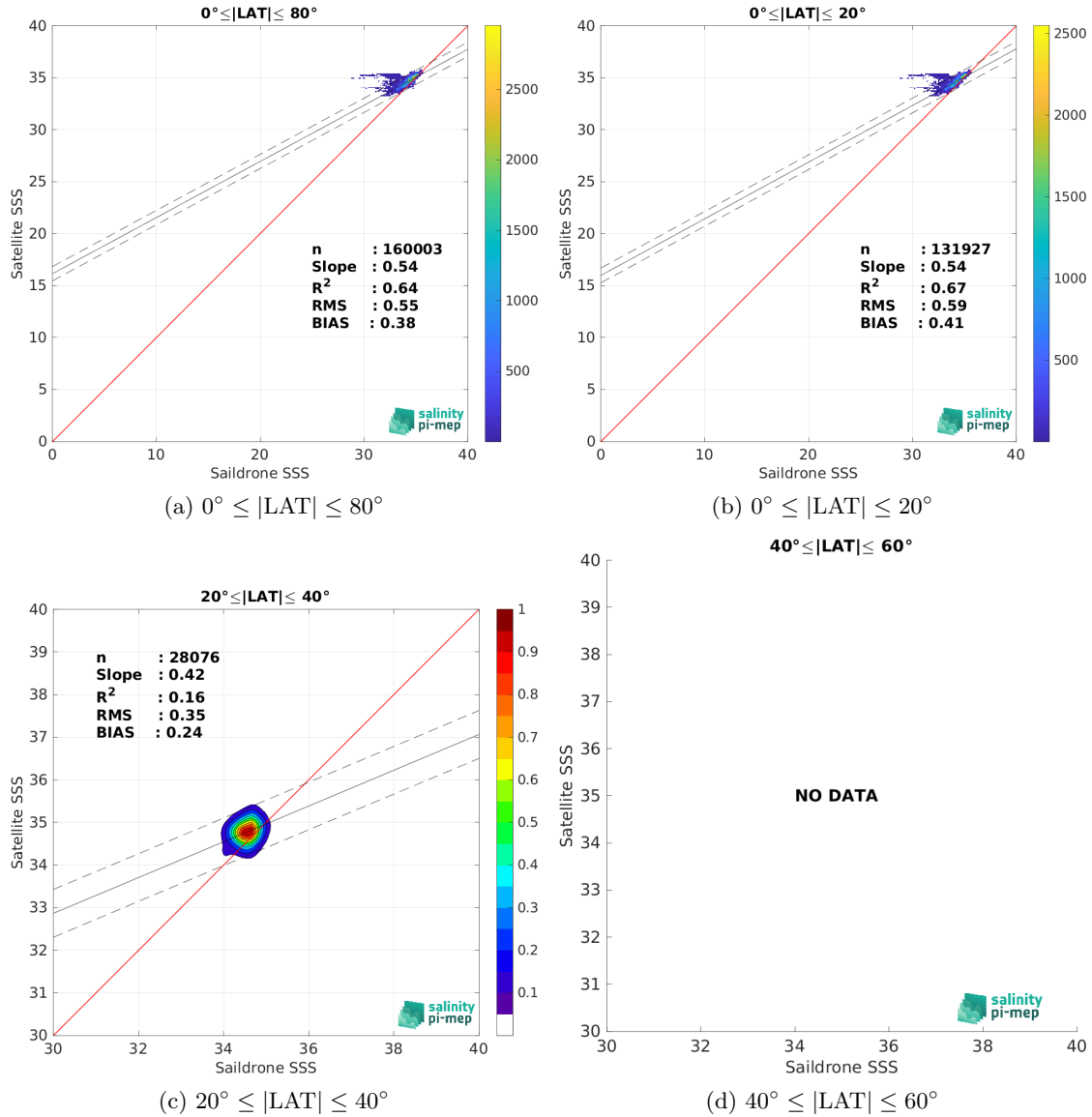
Figure 9: Contour maps of the concentration of SMOS SSS L3 v2 - 9-Days (BEC) SSS (y-axis) versus Sairdrone SSS (x-axis) at match-up pairs for different latitude bands. For each plot, the red line shows x=y . The black thin and dashed lines indicate a linear fit through the data cloud and the \pm 95\% confidence levels, respectively. The number match-up pairs n , the slope and R^2 coefficient of the linear fit, the root mean square (RMS) and the mean bias between satellite and in situ data are indicated for each latitude band in each plots.
