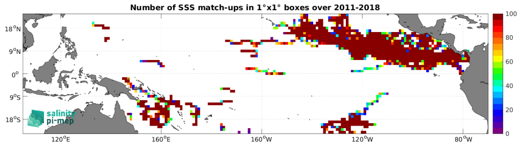
Figure 4: Number of SSS match-ups between Surface drifters SSS and the SMOS SSS L3 v2 - 9-Days (BEC) SSS product for the Tropical Pacific Ocean Pi-MEP region over 1^\circ \times 1^\circ boxes and for the full satellite product period.
