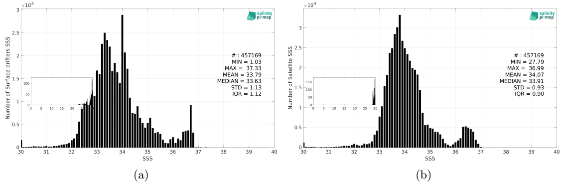
Figure 3: Histograms of SSS from Surface drifters (a) and SMOS SSS L3 v2 - 9-Days (BEC) (b) considering all match-up pairs per bins of 0.1 over the Tropical Pacific Ocean Pi-MEP region and for the full satellite product period.
