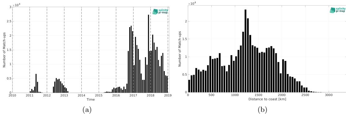
Figure 2: Number of match-ups between Surface drifters and SMOS SSS L3 v2 - 9-Days (BEC) SSS as a function of time (a) and as function of the distance to coast (b) over the Tropical Pacific Ocean Pi-MEP region and for the full satellite product period.
