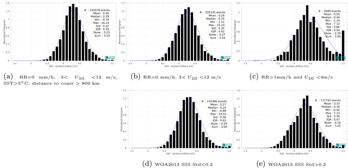
Figure 14: Normalized histogram of \Delta SSS (SMOS SSS L3 v2 - 9-Days (BEC) - Surface drifters) for 5 different subdatasets corresponding to: RR=0 mm/h, 3 < U_{10} < 12 m/s, SST >5^\circ\text{C} , distance to coast > 800 km (a), RR=0 mm/h, 3 < U_{10} < 12 m/s (b), RR >1 mm/h and U_{10} < 4 m/s (c), WOA2013 SSS Std <0.2 (d), WOA2013 SSS Std >0.2 (e).
