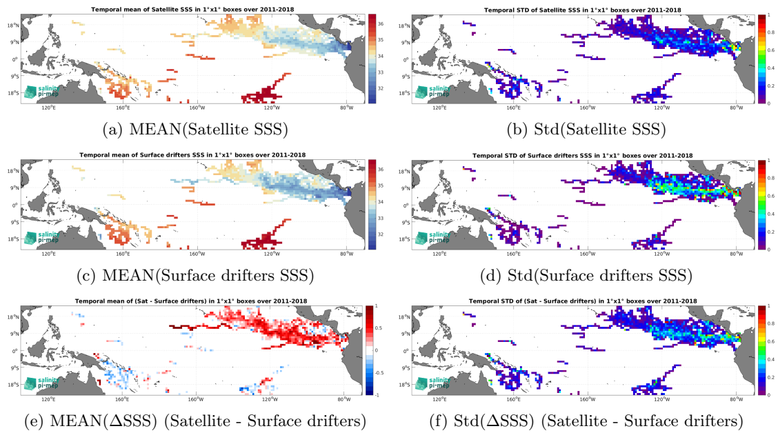
Figure 6: Temporal mean (left) and Std (right) of SSS from SMOS SSS L3 v2 - 9-Days (BEC) (top), Surface drifters (middle), and of \Delta SSS (Satellite - Surface drifters). Only match-up pairs are used to generate these maps.
