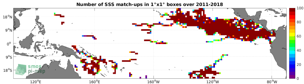
Figure 3: Number of SSS match-ups between Surface drifters SSS and the SMOS SSS L3 v2 - 9-Days (BEC) SSS product for the Tropical Pacific Ocean Pi-MEP region over 1^\circ \times 1^\circ boxes and for the full satellite product period.
