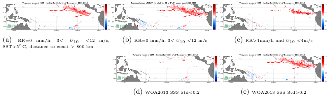
Figure 11: Temporal mean gridded over spatial boxes of size 1°x1° of ΔSSS (SMOS SSS L3 v2 - 9-Days (BEC) - Surface drifters) for 5 different subdatasets corresponding to:RR=0 mm/h, 3 < U_{10} < 12 m/s, SST>5°C, distance to coast > 800 km (a), RR=0 mm/h, 3 < U_{10} < 12 m/s (b), RR>1mm/h and U_{10} < 4m/s (c), WOA2013 SSS Std<0.2 (d), WOA2013 SSS Std>0.2 (e).
