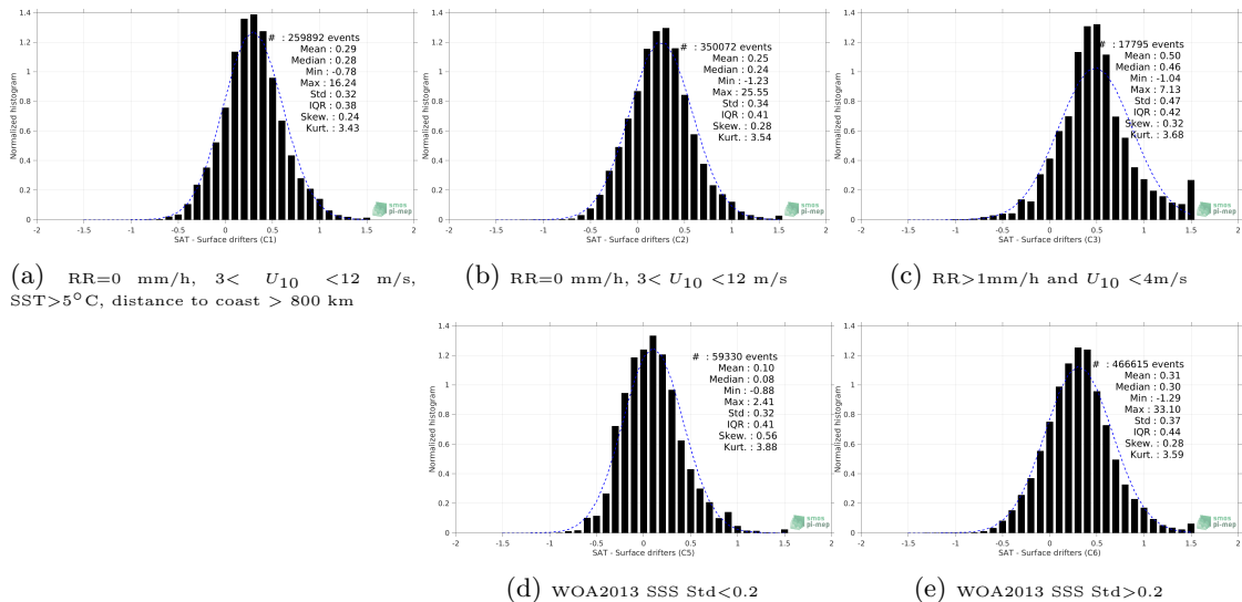
Figure 12: Normalized histogram of ΔSSS (SMOS SSS L3 v2 - 9-Days (BEC) - Surface drifters) for 5 different subdatasets corresponding to: RR=0 mm/h, 3 < U_{10} < 12 m/s, SST>5°C, distance to coast > 800 km (a), RR=0 mm/h, 3 < U_{10} < 12 m/s (b), RR>1mm/h and U_{10} < 4m/s (c), WOA2013 SSS Std<0.2 (d), WOA2013 SSS Std>0.2 (e).
