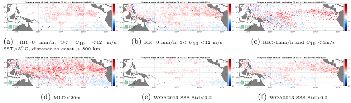
Figure 12: Temporal mean gridded over spatial boxes of size 1^\circ \times 1^\circ of \Delta SSS (SMOS SSS L3 v2 - 9-Days (BEC) - Argo) for 6 different subdatasets corresponding to: RR=0 mm/h, 3 < U_{10} < 12 m/s, SST > 5^\circ C , distance to coast > 800 km (a), RR=0 mm/h, 3 < U_{10} < 12 m/s (b), RR > 1 mm/h and U_{10} < 4 m/s (c), MLD < 20 m (d), WOA2013 SSS Std < 0.2 (e), WOA2013 SSS Std > 0.2 (f).
