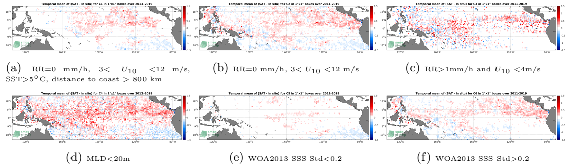
Figure 12: Temporal mean gridded over spatial boxes of size 1^\circ \times 1^\circ of \Delta SSS (SMOS SSS L3 v2 - 9-Days (BEC) - Argo) for 6 different subdatasets corresponding to:RR=0 mm/h, 3 < U_{10} < 12 m/s, SST >5^\circ\text{C} , distance to coast > 800 km (a), RR=0 mm/h, 3 < U_{10} < 12 m/s (b), RR >1 mm/h and U_{10} < 4 m/s (c),MLD <20 m (d),WOA2013 SSS Std <0.2 (e),WOA2013 SSS Std >0.2 (f).
