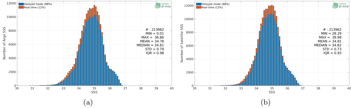
Figure 2: Histograms of SSS from Argo (a) and SMOS SSS L3 v2 - 9-Days (BEC) (b) considering all match-up pairs per bins of 0.1 over the Tropical Pacific Ocean Pi-MEP region and for the full satellite product period.
