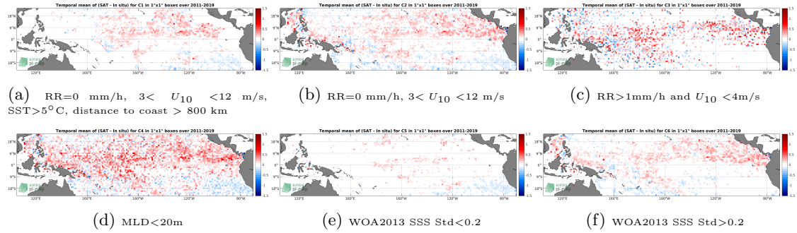
Figure 12: Temporal mean gridded over spatial boxes of size 1^\circ \times 1^\circ of \Delta SSS (SMOS SSS L3 v2 - 9-Days (BEC) - Argo) for 6 different subdatasets corresponding to: RR=0 mm/h, 3 < U_{10} < 12 m/s, SST > 5^\circ C , distance to coast > 800 km (a), RR=0 mm/h, 3 < U_{10} < 12 m/s (b), RR > 1 mm/h and U_{10} < 4 m/s (c), MLD < 20 m (d), WOA2013 SSS Std < 0.2 (e), WOA2013 SSS Std > 0.2 (f).
