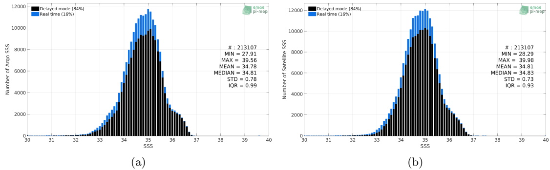
Figure 2: Histograms of SSS from Argo (a) and SMOS L3 v2 - 9-Days (BEC) (b) considering all match-up pairs per bins of 0.1 over the Tropical Pacific Ocean Pi-MEP region and for the full satellite product period.
