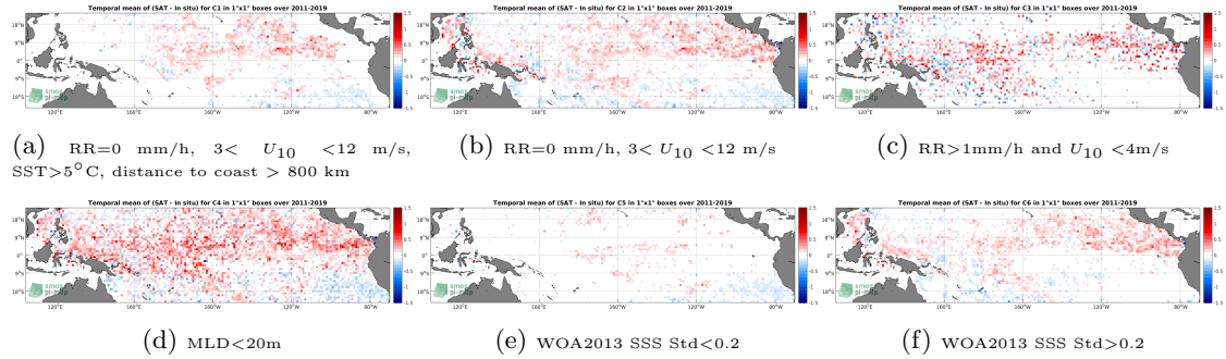
Figure 12: Temporal mean gridded over spatial boxes of size 1^\circ \times 1^\circ of \Delta SSS (SMOS L3 v2 - 9-Days (BEC) - Argo) for 6 different subdatasets corresponding to: RR=0 mm/h, 3 < U_{10} < 12 m/s, SST > 5^\circ C , distance to coast > 800 km (a), RR=0 mm/h, 3 < U_{10} < 12 m/s (b), RR > 1 mm/h and U_{10} < 4 m/s (c), MLD < 20 m (d), WOA2013 SSS Std < 0.2 (e), WOA2013 SSS Std > 0.2 (f).
