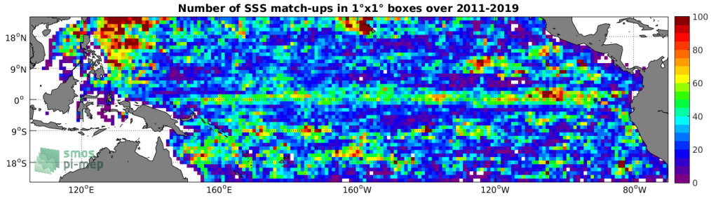
Figure 4: Number of SSS match-ups between Argo SSS and the SMOS L3 v2 - 9-Days (BEC) SSS product for the Tropical Pacific Ocean Pi-MEP region over 1^\circ \times 1^\circ boxes and for the full satellite product period.
