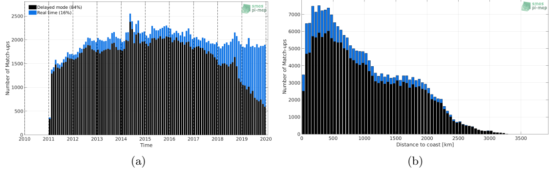
Figure 1: Number of match-ups between Argo and SMOS L3 v2 - 9-Days (BEC) SSS as a function of time (a) and as function of the distance to coast (b) over the Tropical Pacific Ocean Pi-MEP region and for the full satellite product period.
