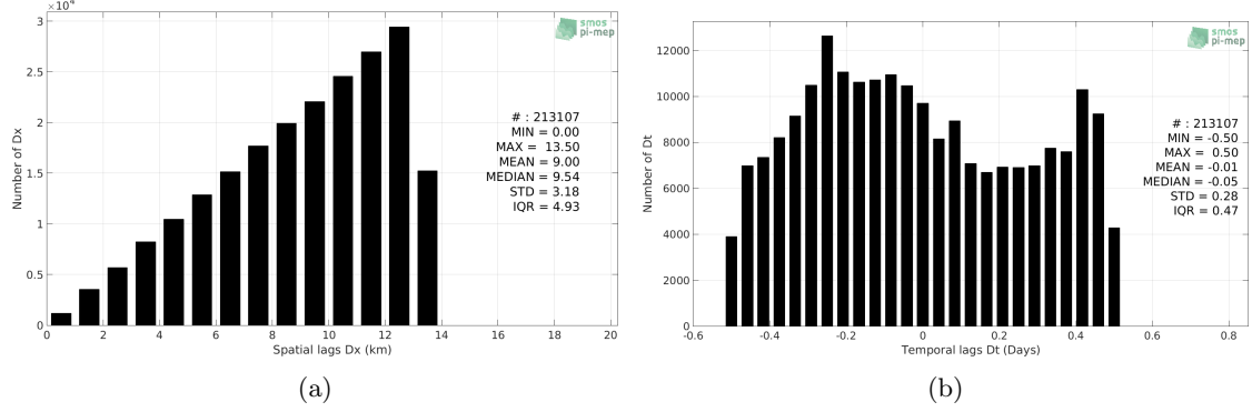
Figure 5: Histograms of the spatial (a) and temporal (b) lags between the time of the Argo measurements and the date of the corresponding SMOS L3 v2 - 9-Days (BEC) SSS product.
