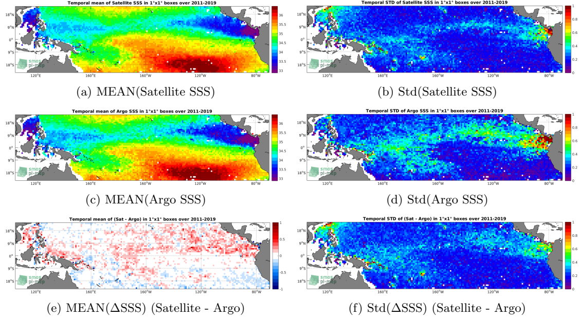
Figure 6: Temporal mean (left) and Std (right) of SSS from SMOS L3 v2 - 9-Days (BEC) (top), Argo (middle), and of \Delta SSS (Satellite - Argo). Only match-up pairs are used to generate these maps.
