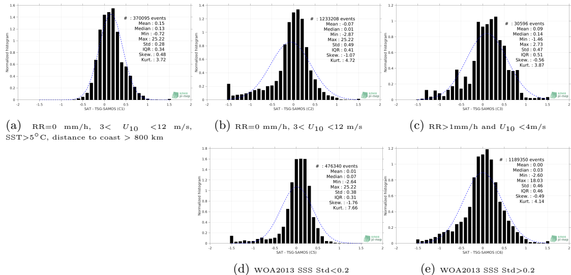
Figure 13: Normalized histogram of \Delta SSS (SMOS-L3-BEC-OA-V1-9DAYS-0.25DEG - TSG-SAMOS) for 5 different subdatasets corresponding to: RR=0 mm/h, 3 < U_{10} < 12 m/s, SST > 5^\circ\text{C} , distance to coast > 800 km (a), RR=0 mm/h, 3 < U_{10} < 12 m/s (b), RR > 1 mm/h and U_{10} < 4 m/s (c), WOA2013 SSS Std < 0.2 (d), WOA2013 SSS Std > 0.2 (e).
