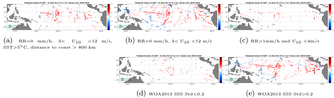
Figure 12: Temporal mean gridded over spatial boxes of size 1^\circ \times 1^\circ of \Delta SSS (SMOS-L3-BEC-OA-V1-9DAYS-0.25DEG - TSG-SAMOS) for 5 different subdatasets corresponding to: RR=0 mm/h, 3 < U_{10} < 12 m/s, SST > 5^\circ\text{C} , distance to coast > 800 km (a), RR=0 mm/h, 3 < U_{10} < 12 m/s (b), RR > 1 mm/h and U_{10} < 4 m/s (c), WOA2013 SSS Std < 0.2 (d), WOA2013 SSS Std > 0.2 (e).
