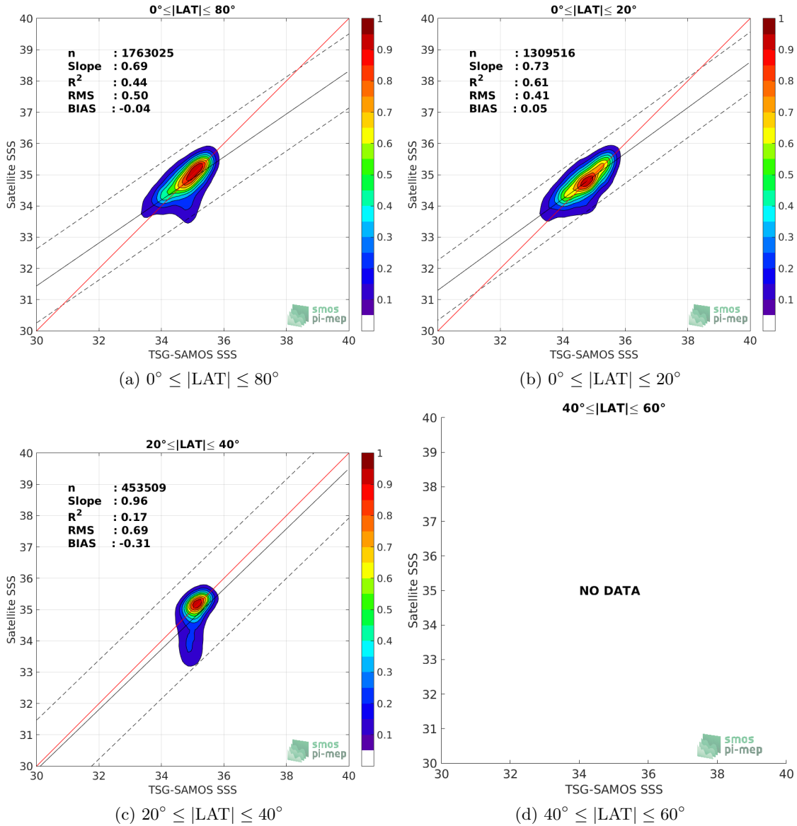
Figure 9: Contour maps of the concentration of SMOS-L3-BEC-OA-V1-9DAYS-0.25DEG SSS (y-axis) versus TSG-SAMOS SSS (x-axis) at match-up pairs for different latitudinal bands. For each plot, the red line shows x=y . The black thin and dashed lines indicate a linear fit through the data cloud and the \pm 95\% confidence levels, respectively. The number match-up pairs n , the slope and R^2 coefficient of the linear fit, the root mean square (RMS) and the mean bias between satellite and in situ data are indicated for each latitude band in each plots.
