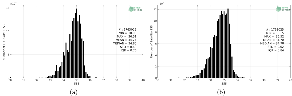
Figure 2: Histograms of SSS from TSG-SAMOS (a) and SMOS-L3-BEC-OA-V1-9DAYS-0.25DEG (b) considering all match-up pairs per bins of 0.1 over the Tropical Pacific Ocean Pi-MEP region and for the full satellite product period.
