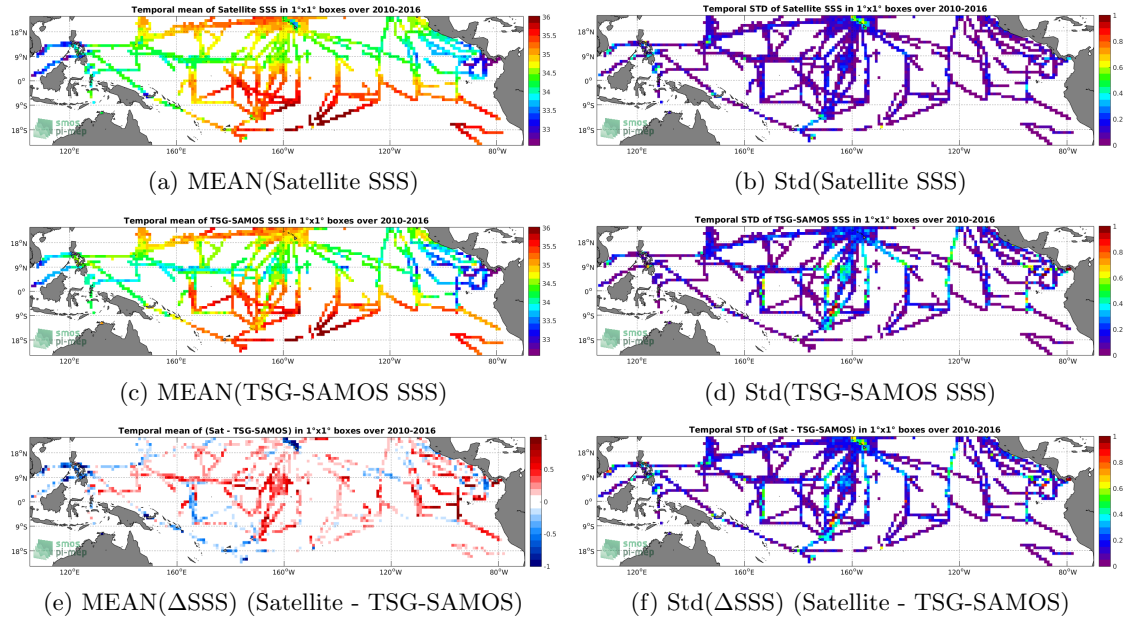
Figure 6: Temporal mean (left) and Std (right) of SSS from SMOS-L3-BEC-OA-V1-9DAYS-0.25DEG (top), TSG-SAMOS (middle), and of \Delta SSS (Satellite - TSG-SAMOS). Only match-up pairs are used to generate these maps.
