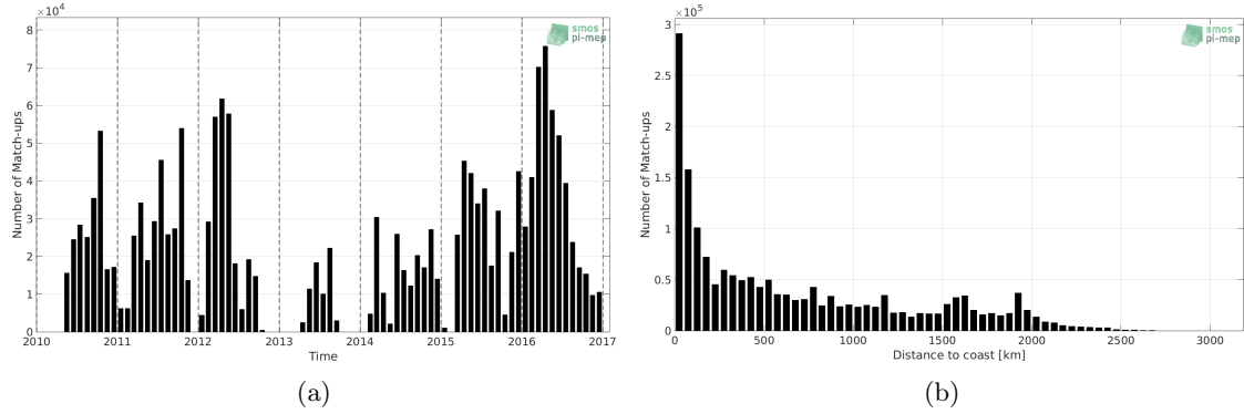
Figure 1: Number of match-ups between TSG-SAMOS and SMOS-L3-BEC-OA-V1-9DAYS-0.25DEG SSS as a function of time (a) and as function of the distance to coast (b) over the Tropical Pacific Ocean Pi-MEP region and for the full satellite product period.
