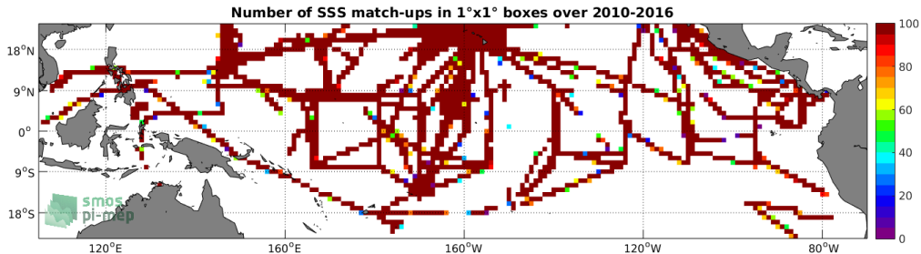
Figure 4: Number of SSS match-ups between TSG-SAMOS SSS and the SMOS-L3-BEC-OA-V1-9DAYS-0.25DEG SSS product for the Tropical Pacific Ocean Pi-MEP region over 1^\circ \times 1^\circ boxes and for the full satellite product period.
