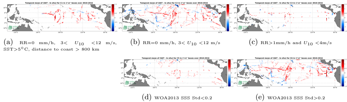
Figure 12: Temporal mean gridded over spatial boxes of size 1^\circ \times 1^\circ of \Delta SSS (SMOS-L3-BEC-OA-V1-9DAYS-0.25DEG - TSG-SAMOS) for 5 different subdatasets corresponding to:RR=0 mm/h, 3 < U_{10} < 12 m/s, SST >5^\circ C, distance to coast > 800 km (a), RR=0 mm/h, 3 < U_{10} < 12 m/s (b), RR >1 mm/h and U_{10} < 4 m/s (c), WOA2013 SSS Std <0.2 (d), WOA2013 SSS Std >0.2 (e).
