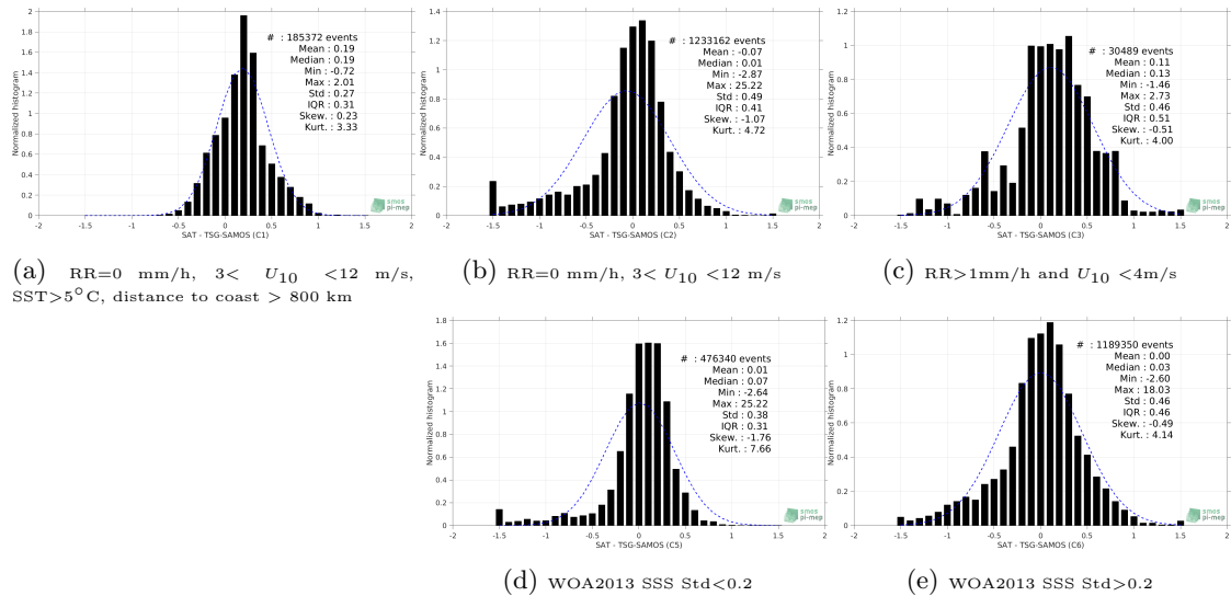
Figure 13: Normalized histogram of \Delta SSS (SMOS-L3-BEC-OA-V1-9DAYS-0.25DEG - TSG-SAMOS) for 5 different subdatasets corresponding to: RR=0 mm/h, 3 < U_{10} < 12 m/s, SST >5^\circ C, distance to coast > 800 km (a), RR=0 mm/h, 3 < U_{10} < 12 m/s (b), RR >1 mm/h and U_{10} < 4 m/s (c), WOA2013 SSS Std <0.2 (d), WOA2013 SSS Std >0.2 (e).
