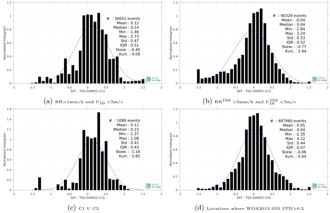
Figure 13: Normalized histogram of \Delta\text{SSS} (SMOS-L3-BEC-OA-V1-9DAYS-0.25DEG - TSG-SAMOS) for 6 different subdatasets corresponding to: RR > 1mm/h and U_{10} < 5\text{m/s} (a), RR^{10d} > 5\text{mm/h} and U_{10}^{10d} < 5\text{m/s} (b), C1 U C2 (c), Locations where WOA2013 SSS STD > 0.2 (d).
