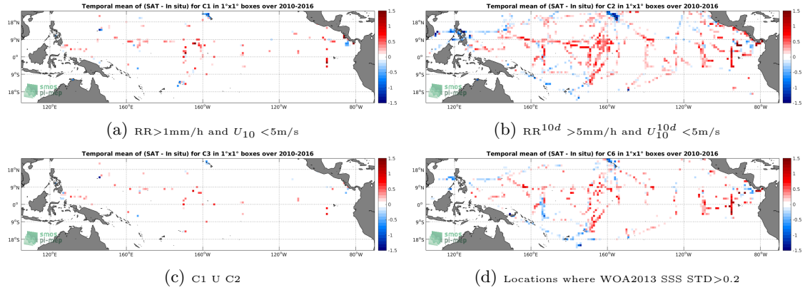
Figure 12: Temporal mean gridded over spatial boxes of size 1^\circ \times 1^\circ of \Delta SSS (SMOS-L3-BEC-OA-V1-9DAYS-0.25DEG - TSG-SAMOS) for 4 different subdatasets corresponding to: RR > 1mm/h and U_{10} < 5\text{m/s} (a), RR^{10d} > 5\text{mm/h} and U_{10}^{10d} < 5\text{m/s} (b), C1 U C2 (c), Locations where WOA2013 SSS STD > 0.2 (d).
