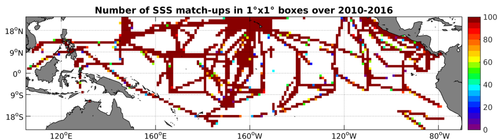
Figure 4: Number of SSS match-ups between TSG-SAMOS SSS and the SMOS-L3-BEC-OA-V1-9DAYS-0.25DEG SSS product for the Tropical Pacific Ocean Pi-MEP region over 1^\circ \times 1^\circ boxes and for the full satellite product period.
