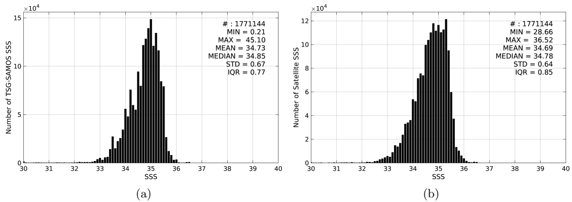
Figure 2: Histograms of SSS from TSG-SAMOS (a) and SMOS-L3-BEC-OA-V1-9DAYS-0.25DEG (b) considering all match-up pairs per bins of 0.1 over the Tropical Pacific Ocean Pi-MEP region and for the full satellite product period.
