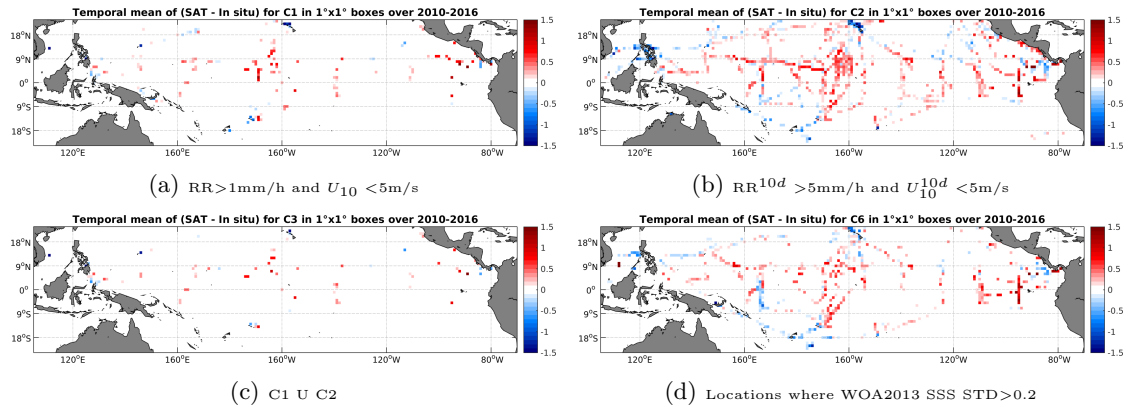
Figure 12: Temporal mean gridded over spatial boxes of size 1^\circ \times 1^\circ of \Delta SSS (SMOS-L3-BEC-OA-V1-9DAYS-0.25DEG - TSG-SAMOS) for 4 different subdatasets corresponding to: RR > 1\text{mm/h} and U_{10} < 5\text{m/s} (a), RR^{10d} > 5\text{mm/h} and U_{10}^{10d} < 5\text{m/s} (b), C1 U C2 (c), Locations where WOA2013 SSS STD > 0.2 (d).
