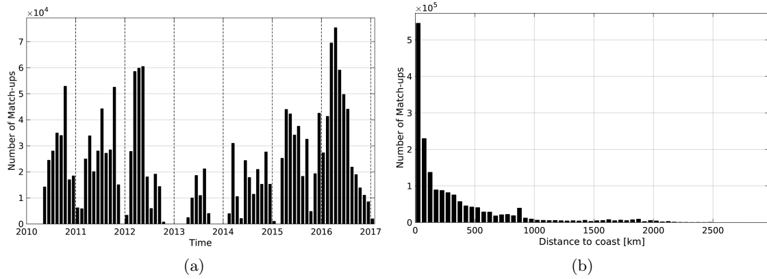
Figure 1: Number of match-ups between TSG-SAMOS and SMOS-L3-BEC-OA-V1-9DAYS-0.25DEG SSS as a function of time (a) and as function of the distance to coast (b) over the Tropical Pacific Ocean Pi-MEP region and for the full satellite product period.
