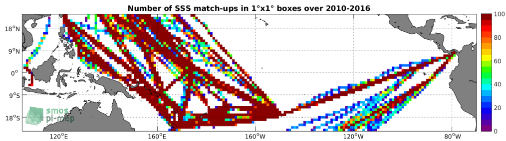
Figure 4: Number of SSS match-ups between TSG-LEGOS-DM SSS and the SMOS-L3-BEC-OA-V1-9DAYS-0.25DEG SSS product for the Tropical Pacific Ocean Pi-MEP region over 1°x1° boxes and for the full satellite product period.
