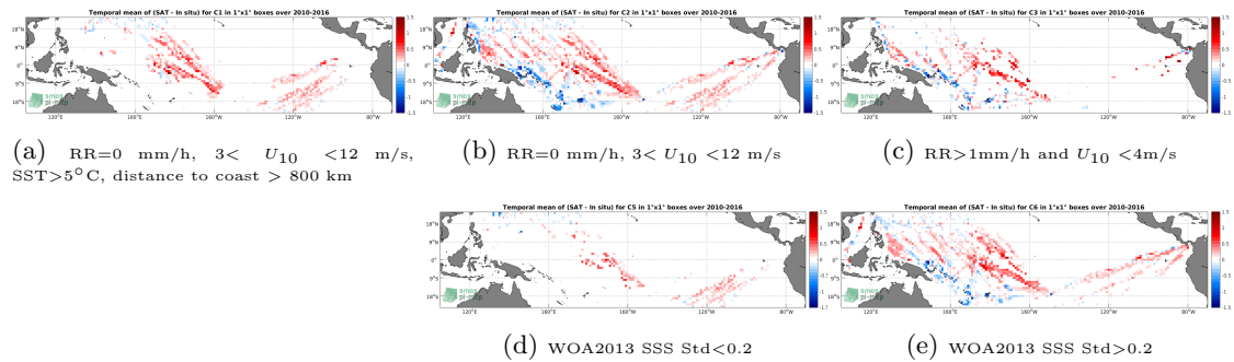
Figure 12: Temporal mean gridded over spatial boxes of size 1^\circ \times 1^\circ of \Delta SSS (SMOS-L3-BEC-OA-V1-9DAYS-0.25DEG - TSG-LEGOS-DM) for 5 different subdatasets corresponding to:RR=0 mm/h, 3 < U_{10} < 12 m/s, SST > 5^\circ\text{C} , distance to coast > 800 km (a), RR=0 mm/h, 3 < U_{10} < 12 m/s (b), RR > 1 mm/h and U_{10} < 4 m/s (c), WOA2013 SSS Std < 0.2 (d), WOA2013 SSS Std > 0.2 (e).
