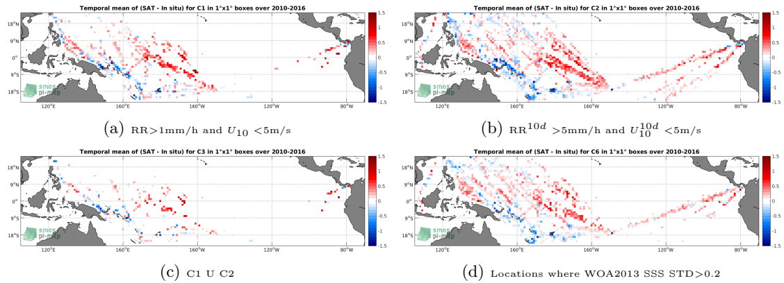
Figure 12: Temporal mean gridded over spatial boxes of size 1^\circ \times 1^\circ of \Delta SSS (SMOS-L3-BEC-OA-V1-9DAYS-0.25DEG - TSG-LEGOS-DM) for 4 different subdatasets corresponding to: RR > 1\text{mm/h} and U_{10} < 5\text{m/s} (a), RR^{10d} > 5\text{mm/h} and U_{10}^{10d} < 5\text{m/s} (b), C1 U C2 (c), Locations where WOA2013 SSS STD > 0.2 (d).
