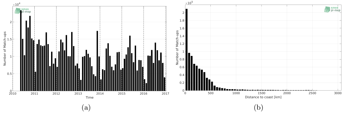
Figure 1: Number of match-ups between TSG-LEGOS-DM and SMOS-L3-BEC-OA-V1-9DAYS-0.25DEG SSS as a function of time (a) and as function of the distance to coast (b) over the Tropical Pacific Ocean Pi-MEP region and for the full satellite product period.
