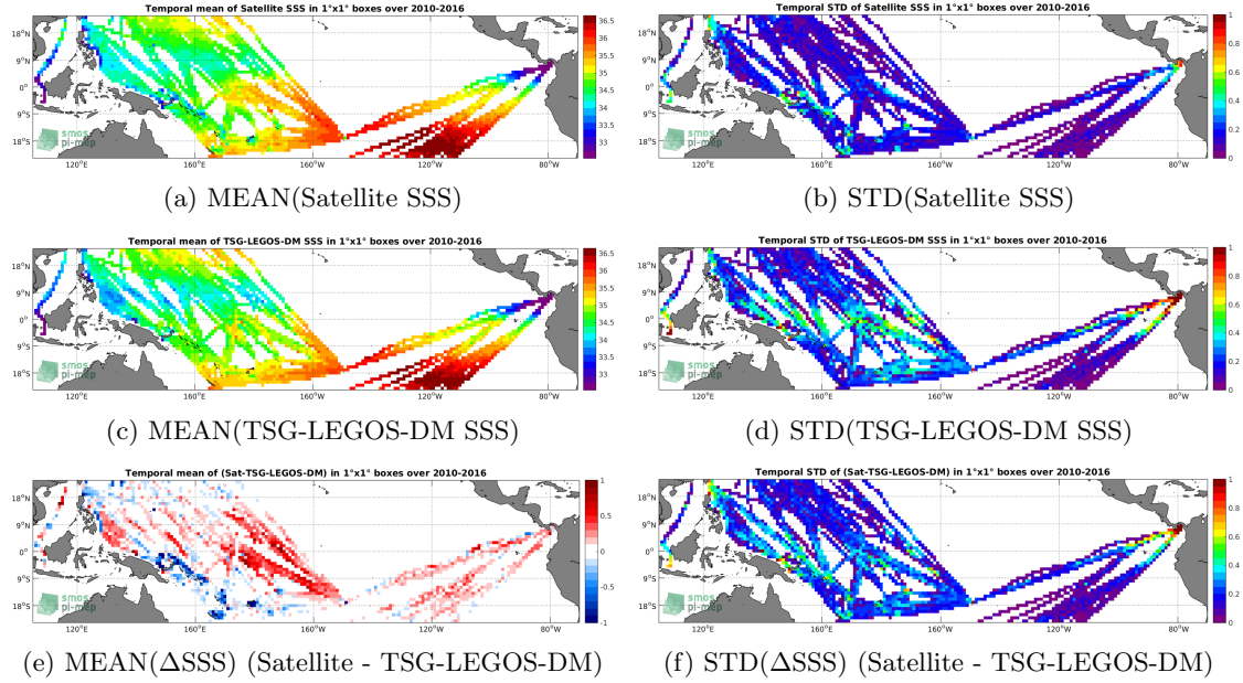
Figure 6: Temporal mean (left) and STD (right) of SSS from SMOS-L3-BEC-OA-V1-9DAYS-0.25DEG (top), TSG-LEGOS-DM (middle), and of \Delta SSS (Satellite - TSG-LEGOS-DM). Only match-up pairs are used to generate these maps.
