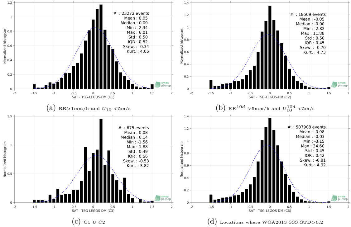
Figure 13: Normalized histogram of \Delta SSS (SMOS-L3-BEC-OA-V1-9DAYS-0.25DEG - TSG-LEGOS-DM) for 6 different subdatasets corresponding to: RR > 1mm/h and U_{10} < 5 m/s (a), RR^{10d} > 5 mm/h and U_{10}^{10d} < 5 m/s (b), C1 U C2 (c), Locations where WOA2013 SSS STD > 0.2 (d).
