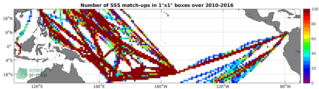
Figure 4: Number of SSS match-ups between TSG-LEGOS-DM SSS and the SMOS-L3-BEC-OA-V1-9DAYS-0.25DEG SSS product for the Tropical Pacific Ocean Pi-MEP region over 1^\circ \times 1^\circ boxes and for the full satellite product period.
