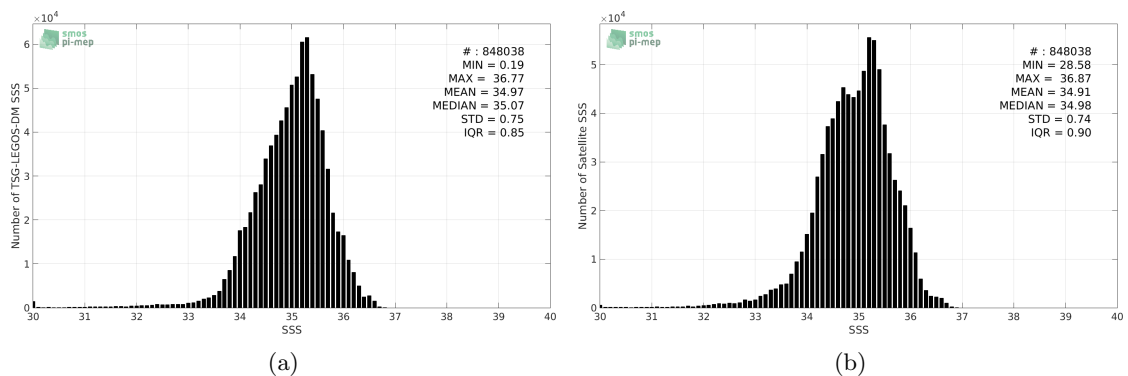
Figure 2: Histograms of SSS from TSG-LEGOS-DM (a) and SMOS-L3-BEC-OA-V1-9DAYS-0.25DEG (b) considering all match-up pairs per bins of 0.1 over the Tropical Pacific Ocean Pi-MEP region and for the full satellite product period.
