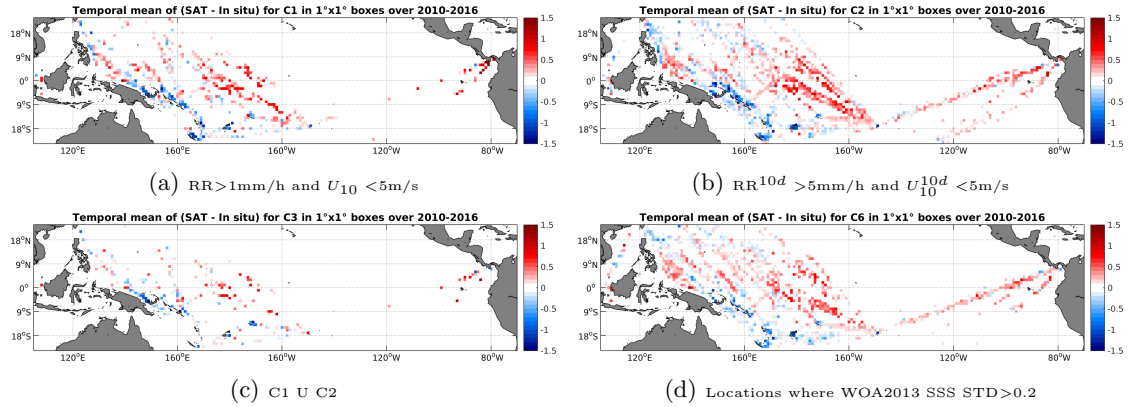
Figure 12: Temporal mean gridded over spatial boxes of size 1^\circ \times 1^\circ of \Delta SSS (SMOS-L3-BEC-OA-V1-9DAYS-0.25DEG - TSG-LEGOS-DM) for 4 different subdatasets corresponding to: RR > 1 mm/h and U_{10} < 5 m/s (a), RR ^{10d} > 5 mm/h and U_{10}^{10d} < 5 m/s (b), C1 U C2 (c), Locations where WOA2013 SSS STD > 0.2 (d).
