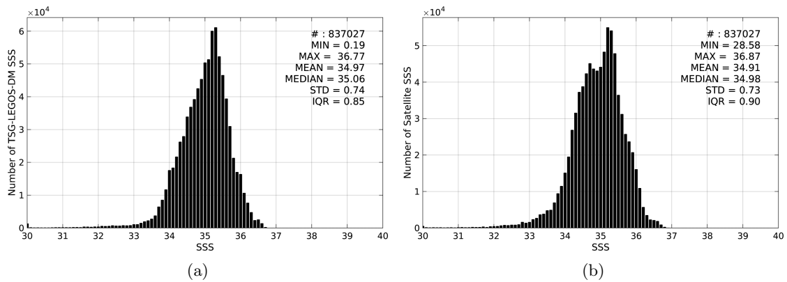
Figure 2: Histograms of SSS from TSG-LEGOS-DM (a) and SMOS-L3-BEC-OA-V1-9DAYS-0.25DEG (b) considering all match-up pairs per bins of 0.1 over the Tropical Pacific Ocean Pi-MEP region and for the full satellite product period.
